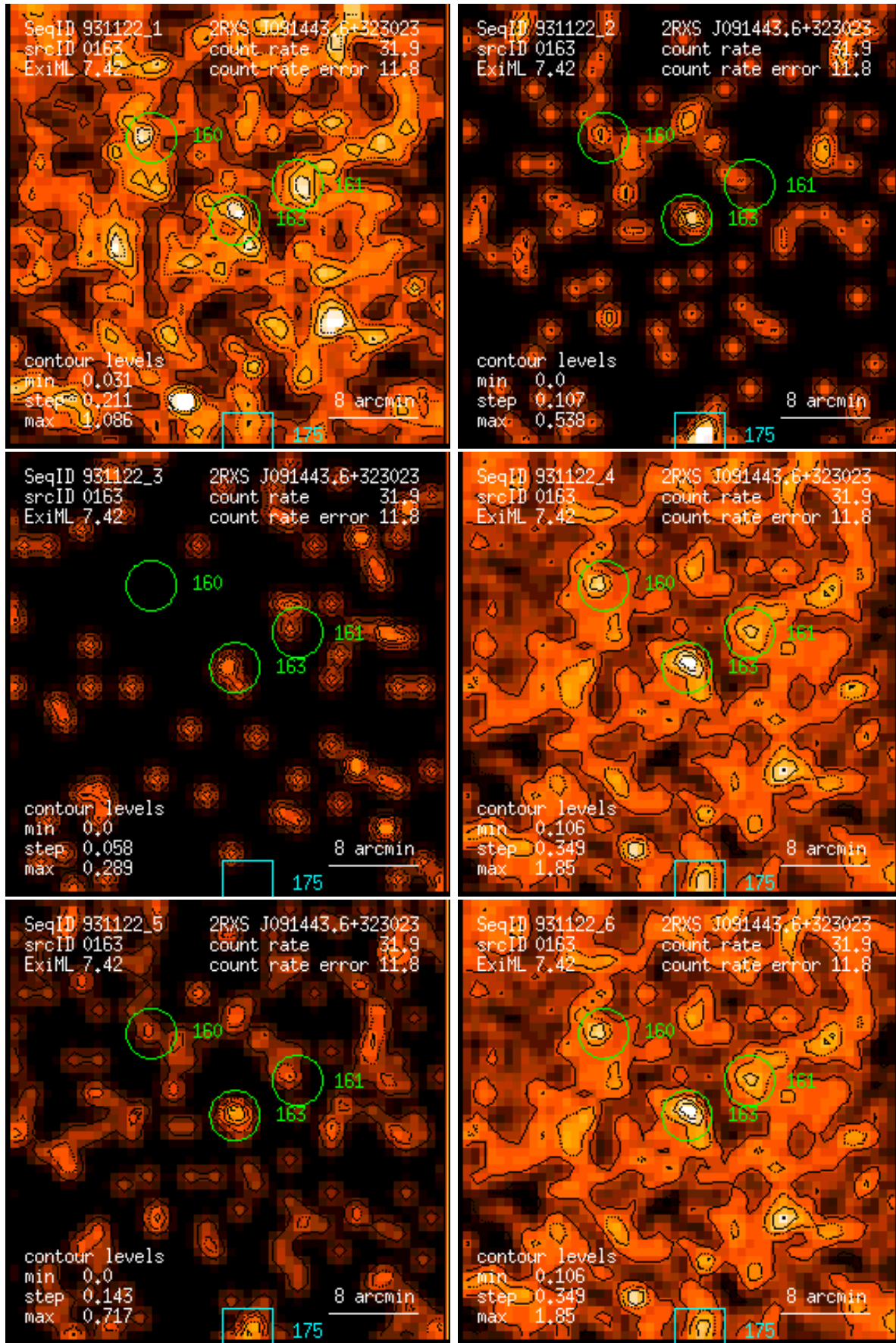
Figure 163: RASS 931122: detection 0163: band rate images, Gaussian filter: (1) PSPC channels 11 – 41, (2) 52 – 90, (3) 91 – 201, (4) 11 – 235, (5) 52 – 201, (6) 11 – 201. Broad band rates in counts/ks. Band rate contour levels in counts/ks/arcmin 2 .
