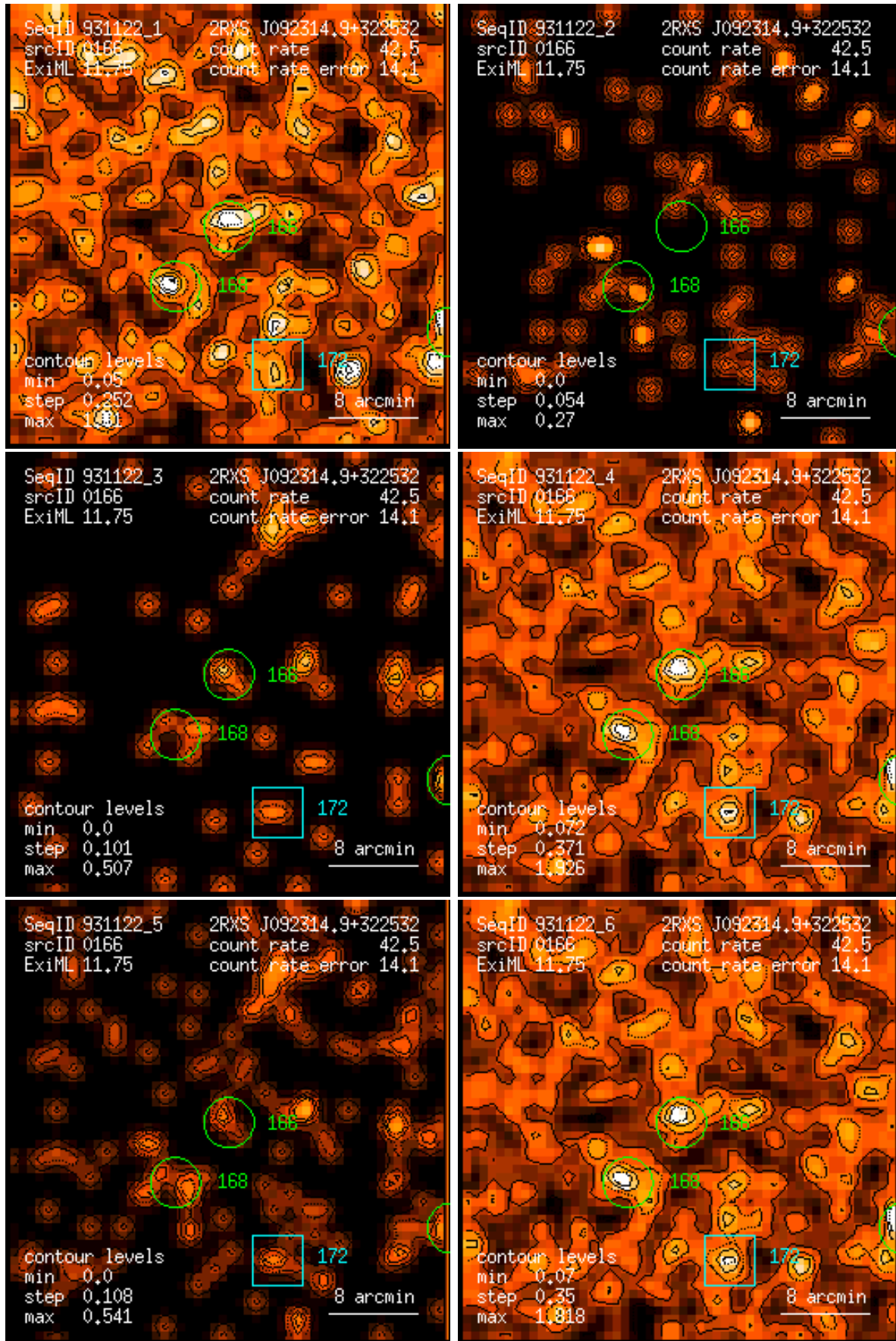
Figure 166: RASS 931122: detection 0166: band rate images, Gaussian filter: (1) PSPC channels 11 – 41, (2) 52 – 90, (3) 91 – 201, (4) 11 – 235, (5) 52 – 201, (6) 11 – 201. Broad band rates in counts/ks. Band rate contour levels in counts/ks/arcmin 2 .
