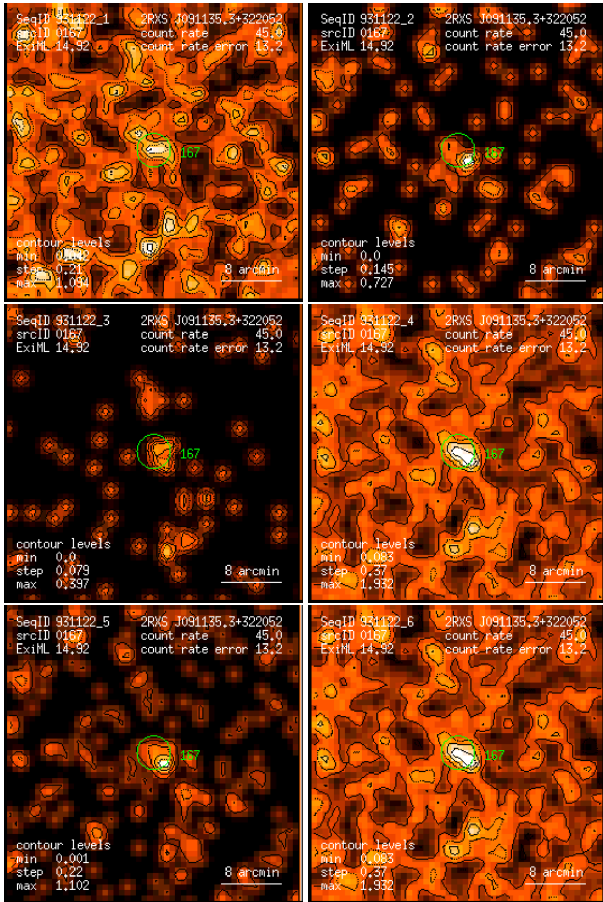
Figure 167: RASS 931122: detection 0167: band rate images, Gaussian filter: (1) PSPC channels 11 – 41, (2) 52 – 90, (3) 91 – 201, (4) 11 – 235, (5) 52 – 201, (6) 11 – 201. Broad band rates in counts/ks. Band rate contour levels in counts/ks/arcmin 2 .
