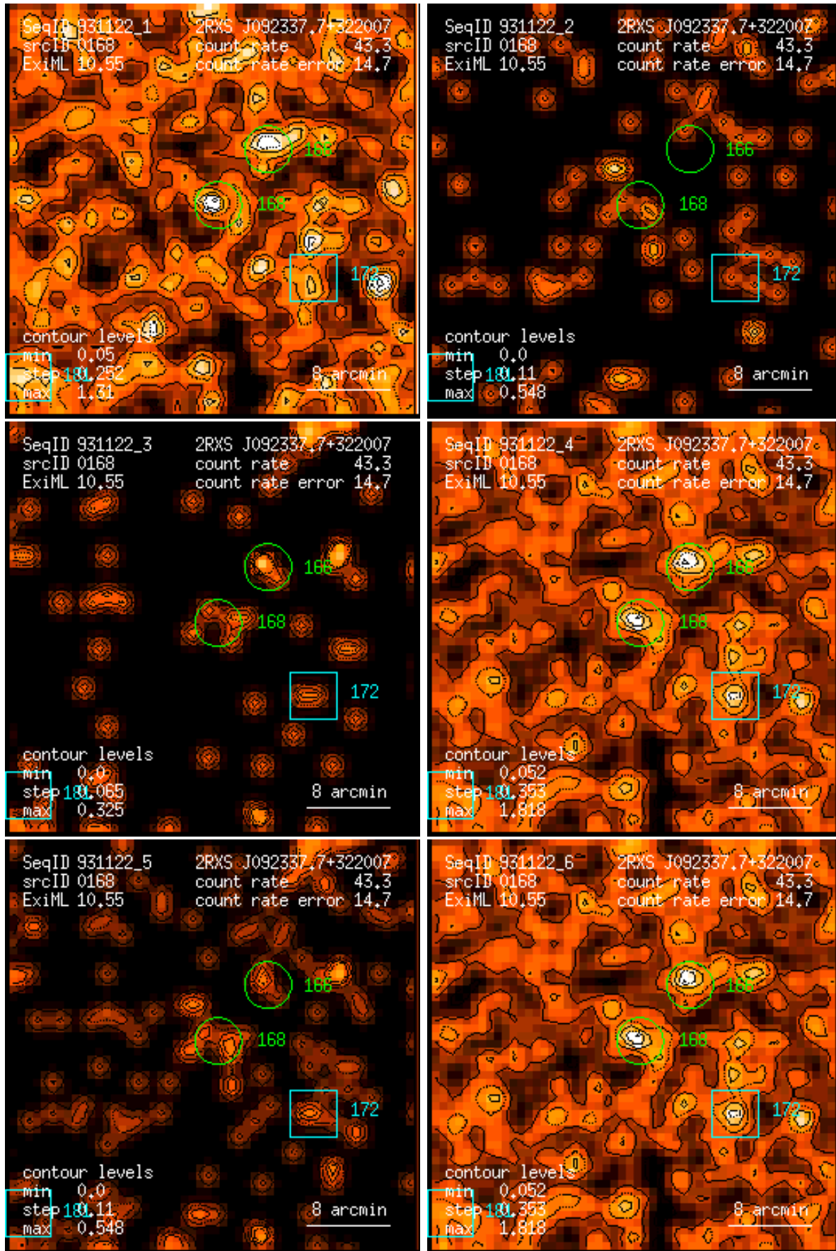
Figure 168: RASS 931122: detection 0168: band rate images, Gaussian filter: (1) PSPC channels 11 – 41, (2) 52 – 90, (3) 91 – 201, (4) 11 – 235, (5) 52 – 201, (6) 11 – 201. Broad band rates in counts/ks. Band rate contour levels in counts/ks/arcmin 2 .
