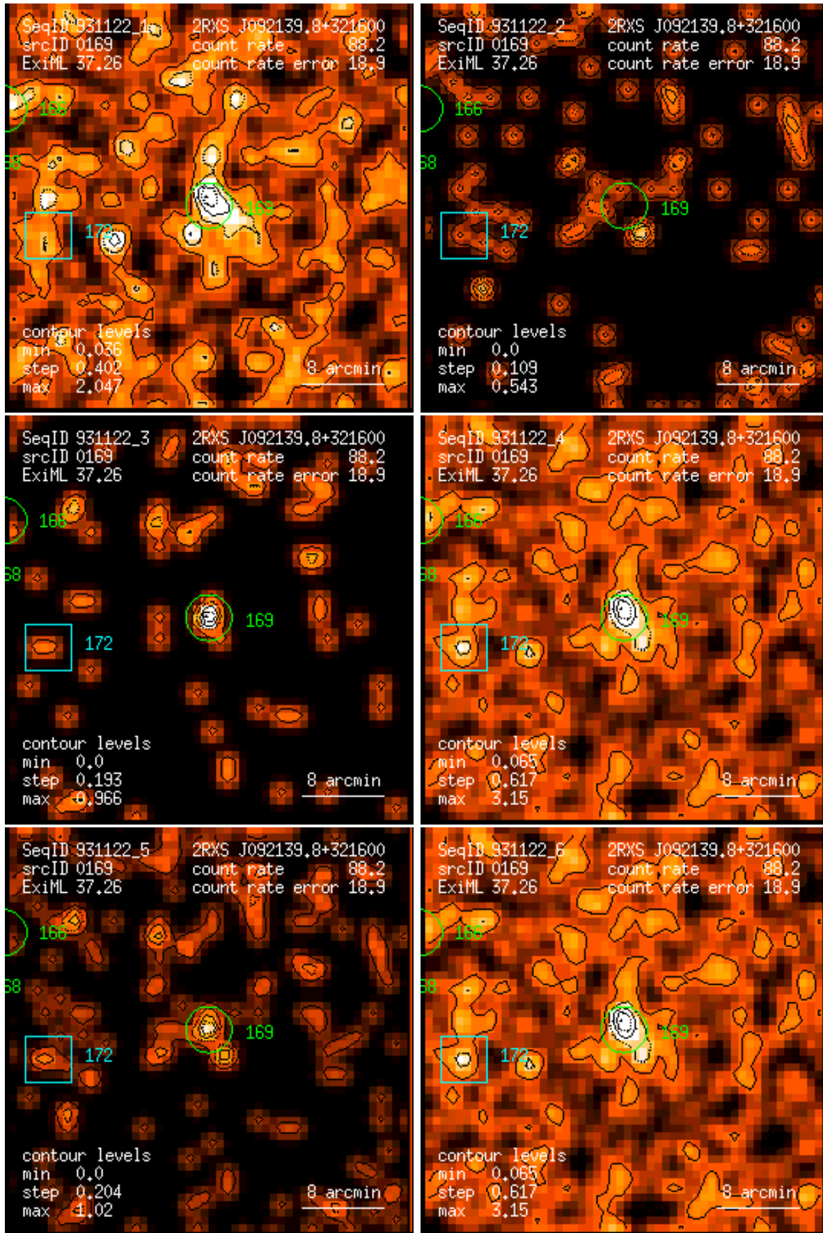
Figure 169: RASS 931122: detection 0169: band rate images, Gaussian filter: (1) PSPC channels 11 – 41, (2) 52 – 90, (3) 91 – 201, (4) 11 – 235, (5) 52 – 201, (6) 11 – 201. Broad band rates in counts/ks. Band rate contour levels in counts/ks/arcmin 2 .
