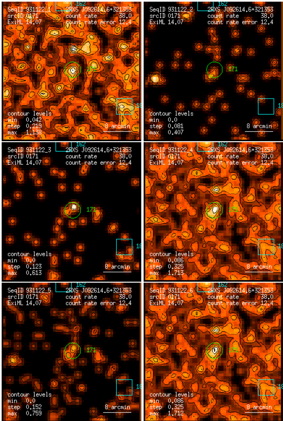
Figure 171: RASS 931122: detection 0171: band rate images, Gaussian filter: (1) PSPC channels 11 – 41, (2) 52 – 90, (3) 91 – 201, (4) 11 – 235, (5) 52 – 201, (6) 11 – 201. Broad band rates in counts/ks. Band rate contour levels in counts/ks/arcmin 2 .
