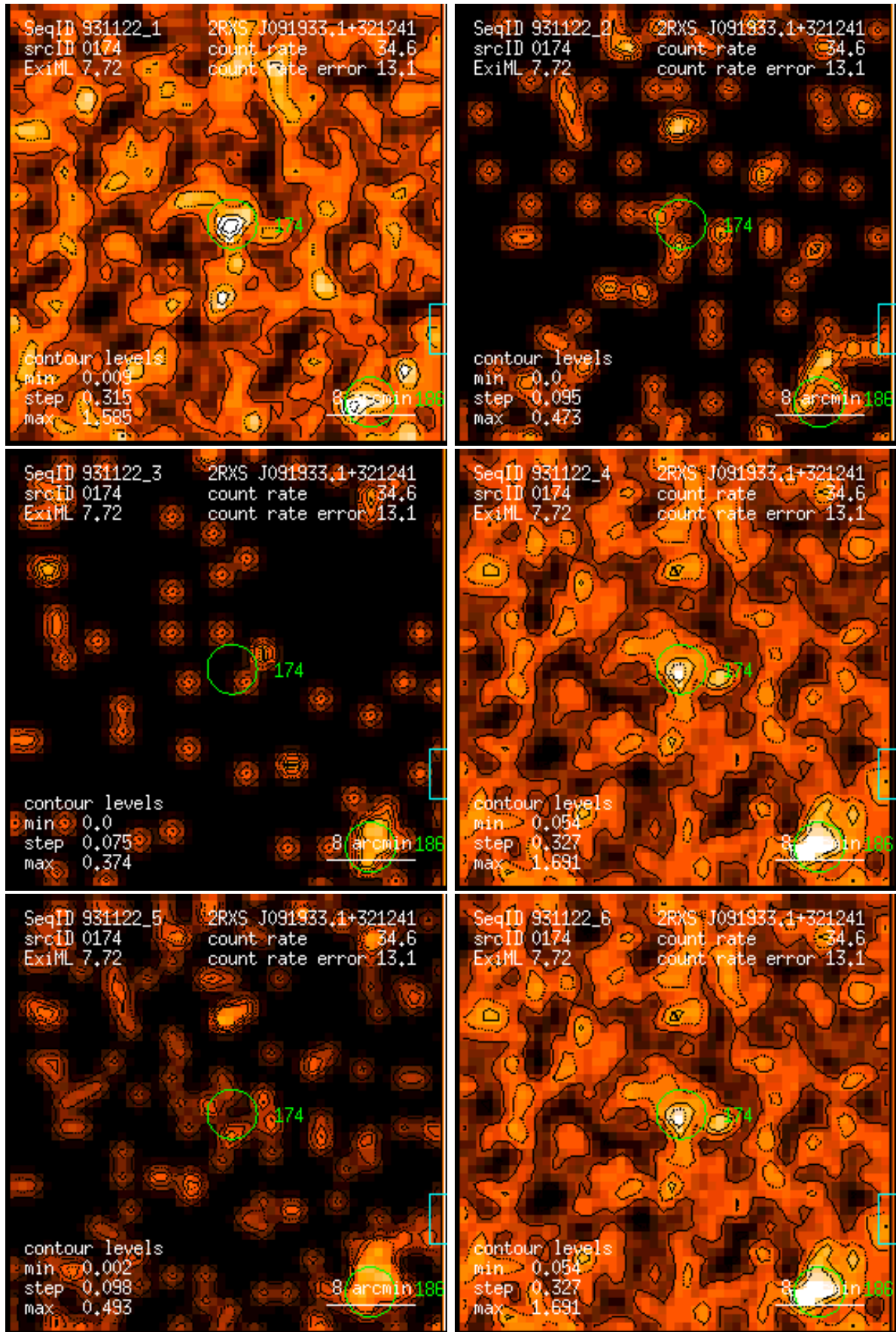
Figure 174: RASS 931122: detection 0174: band rate images, Gaussian filter: (1) PSPC channels 11 – 41, (2) 52 – 90, (3) 91 – 201, (4) 11 – 235, (5) 52 – 201, (6) 11 – 201. Broad band rates in counts/ks. Band rate contour levels in counts/ks/arcmin 2 .
