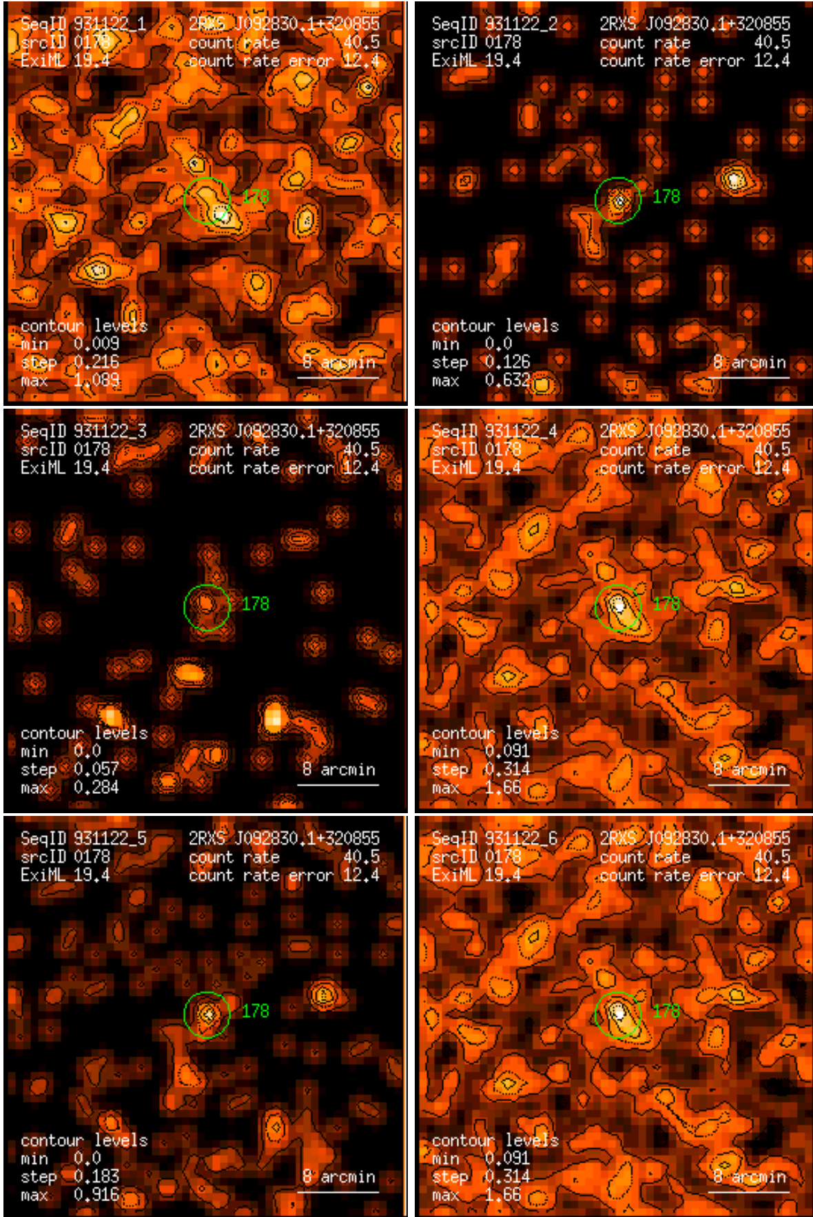
Figure 178: RASS 931122: detection 0178: band rate images, Gaussian filter: (1) PSPC channels 11 – 41, (2) 52 – 90, (3) 91 – 201, (4) 11 – 235, (5) 52 – 201, (6) 11 – 201. Broad band rates in counts/ks. Band rate contour levels in counts/ks/arcmin 2 .
