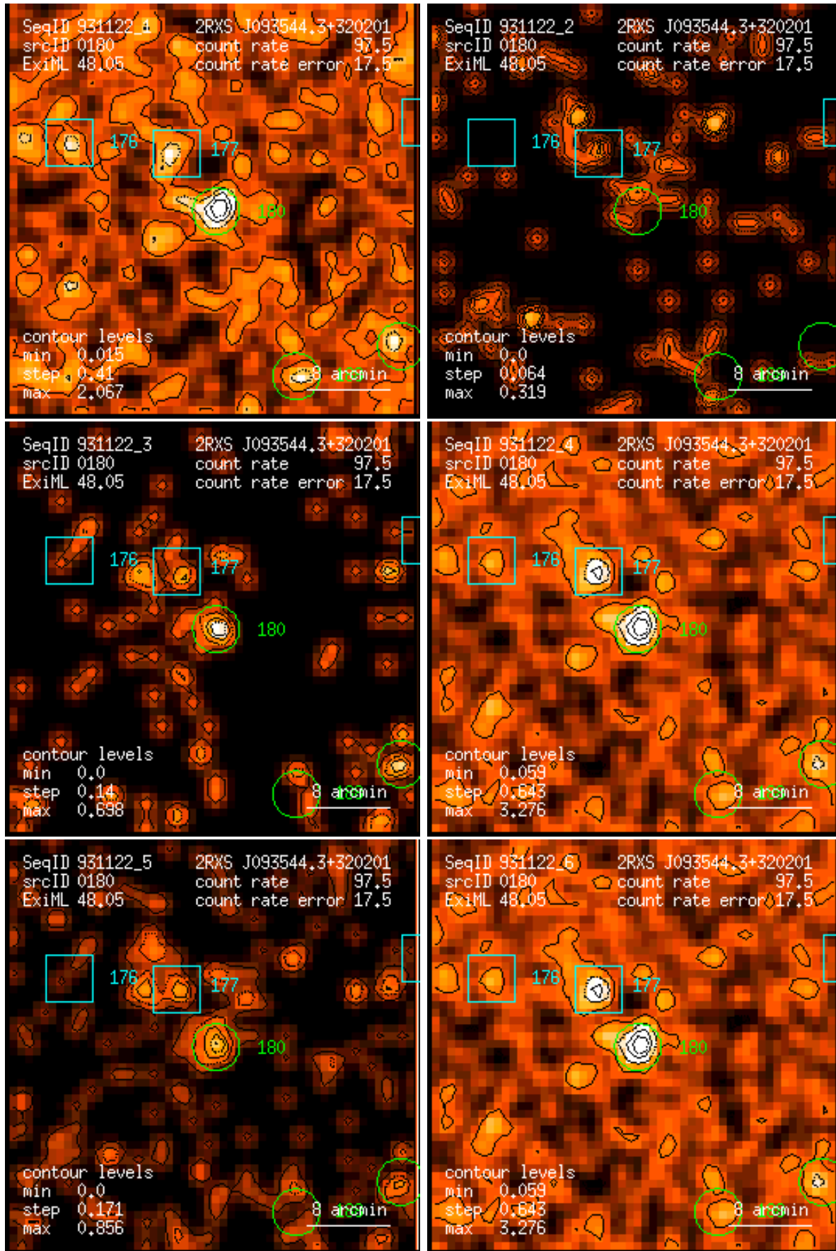
Figure 180: RASS 931122: detection 0180: band rate images, Gaussian filter: (1) PSPC channels 11 – 41, (2) 52 – 90, (3) 91 – 201, (4) 11 – 235, (5) 52 – 201, (6) 11 – 201. Broad band rates in counts/ks. Band rate contour levels in counts/ks/arcmin 2 .
