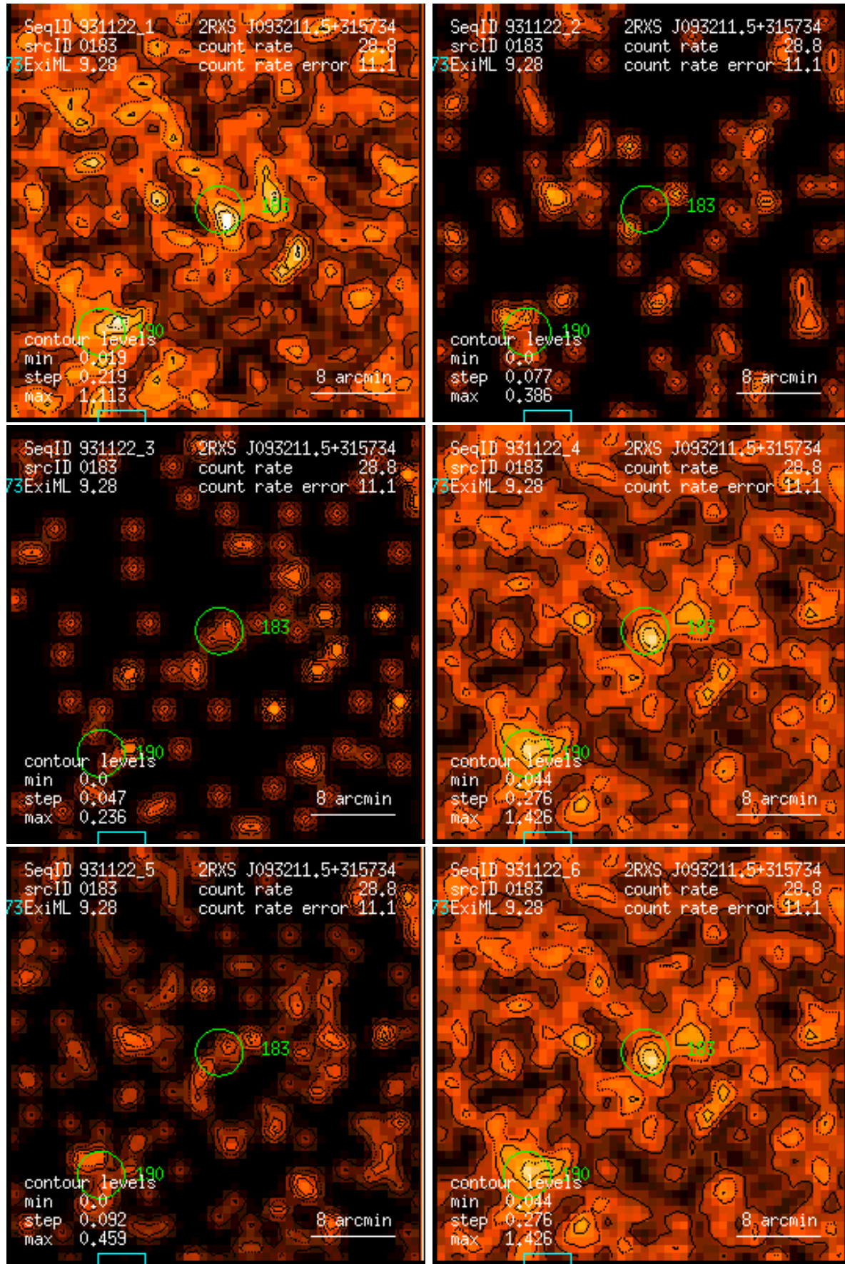
Figure 183: RASS 931122: detection 0183: band rate images, Gaussian filter: (1) PSPC channels 11 – 41, (2) 52 – 90, (3) 91 – 201, (4) 11 – 235, (5) 52 – 201, (6) 11 – 201. Broad band rates in counts/ks. Band rate contour levels in counts/ks/arcmin 2 .
