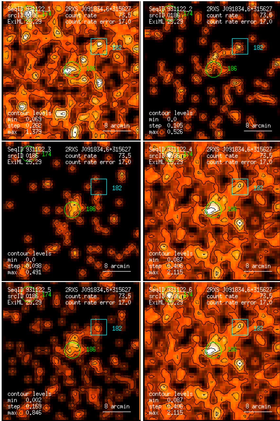
Figure 186: RASS 931122: detection 0186: band rate images, Gaussian filter: (1) PSPC channels 11 – 41, (2) 52 – 90, (3) 91 – 201, (4) 11 – 235, (5) 52 – 201, (6) 11 – 201. Broad band rates in counts/ks. Band rate contour levels in counts/ks/arcmin 2 .
