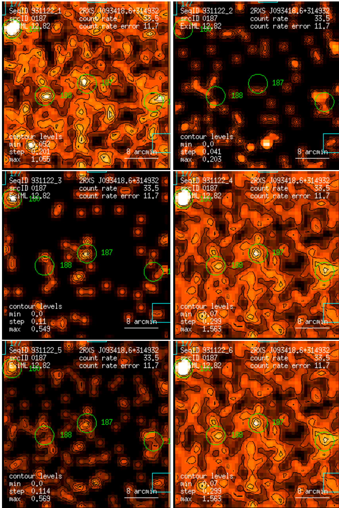
Figure 187: RASS 931122: detection 0187: band rate images, Gaussian filter: (1) PSPC channels 11 – 41, (2) 52 – 90, (3) 91 – 201, (4) 11 – 235, (5) 52 – 201, (6) 11 – 201. Broad band rates in counts/ks. Band rate contour levels in counts/ks/arcmin 2 .
