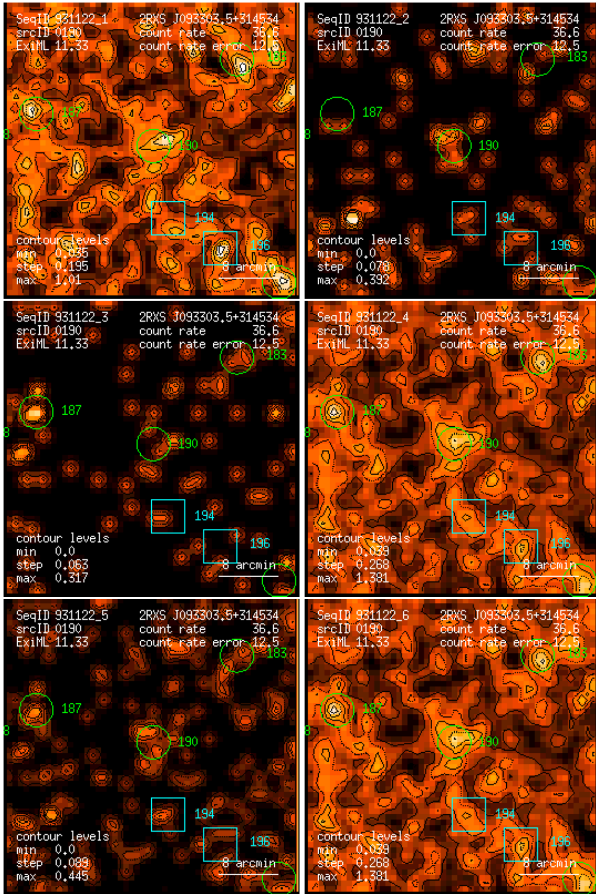
Figure 190: RASS 931122: detection 0190: band rate images, Gaussian filter: (1) PSPC channels 11 – 41, (2) 52 – 90, (3) 91 – 201, (4) 11 – 235, (5) 52 – 201, (6) 11 – 201. Broad band rates in counts/ks. Band rate contour levels in counts/ks/arcmin 2 .
