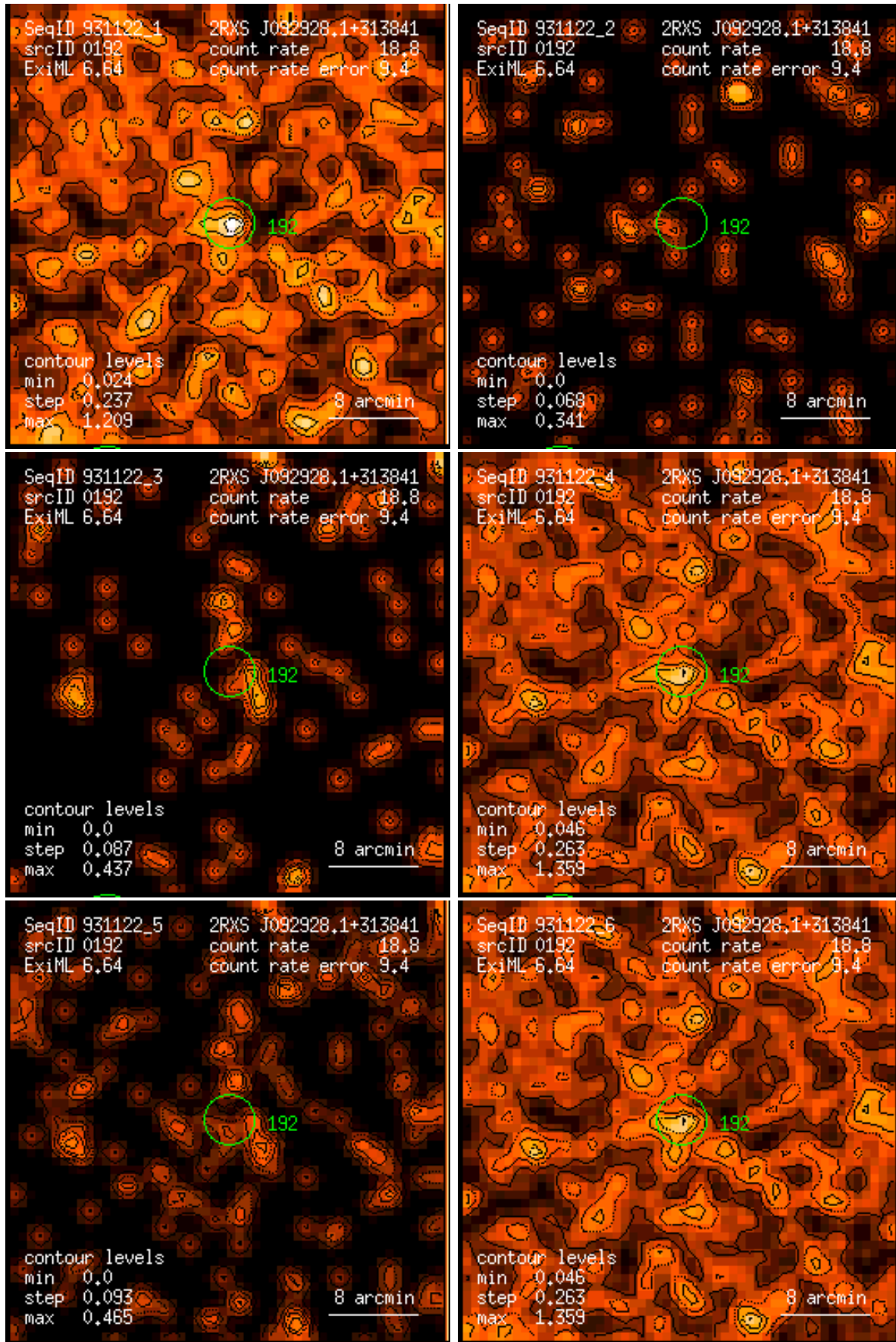
Figure 192: RASS 931122: detection 0192: band rate images, Gaussian filter: (1) PSPC channels 11 – 41, (2) 52 – 90, (3) 91 – 201, (4) 11 – 235, (5) 52 – 201, (6) 11 – 201. Broad band rates in counts/ks. Band rate contour levels in counts/ks/arcmin 2 .
