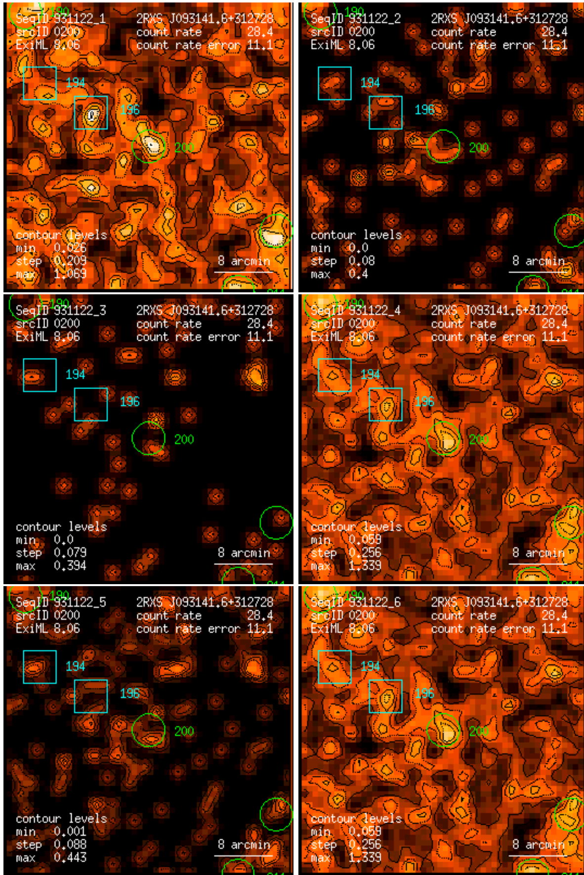
Figure 200: RASS 931122: detection 0200: band rate images, Gaussian filter: (1) PSPC channels 11 – 41, (2) 52 – 90, (3) 91 – 201, (4) 11 – 235, (5) 52 – 201, (6) 11 – 201. Broad band rates in counts/ks. Band rate contour levels in counts/ks/arcmin 2 .
