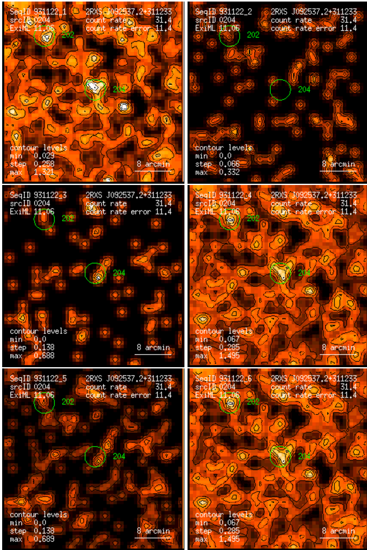
Figure 204: RASS 931122: detection 0204: band rate images, Gaussian filter: (1) PSPC channels 11 – 41, (2) 52 – 90, (3) 91 – 201, (4) 11 – 235, (5) 52 – 201, (6) 11 – 201. Broad band rates in counts/ks. Band rate contour levels in counts/ks/arcmin 2 .
