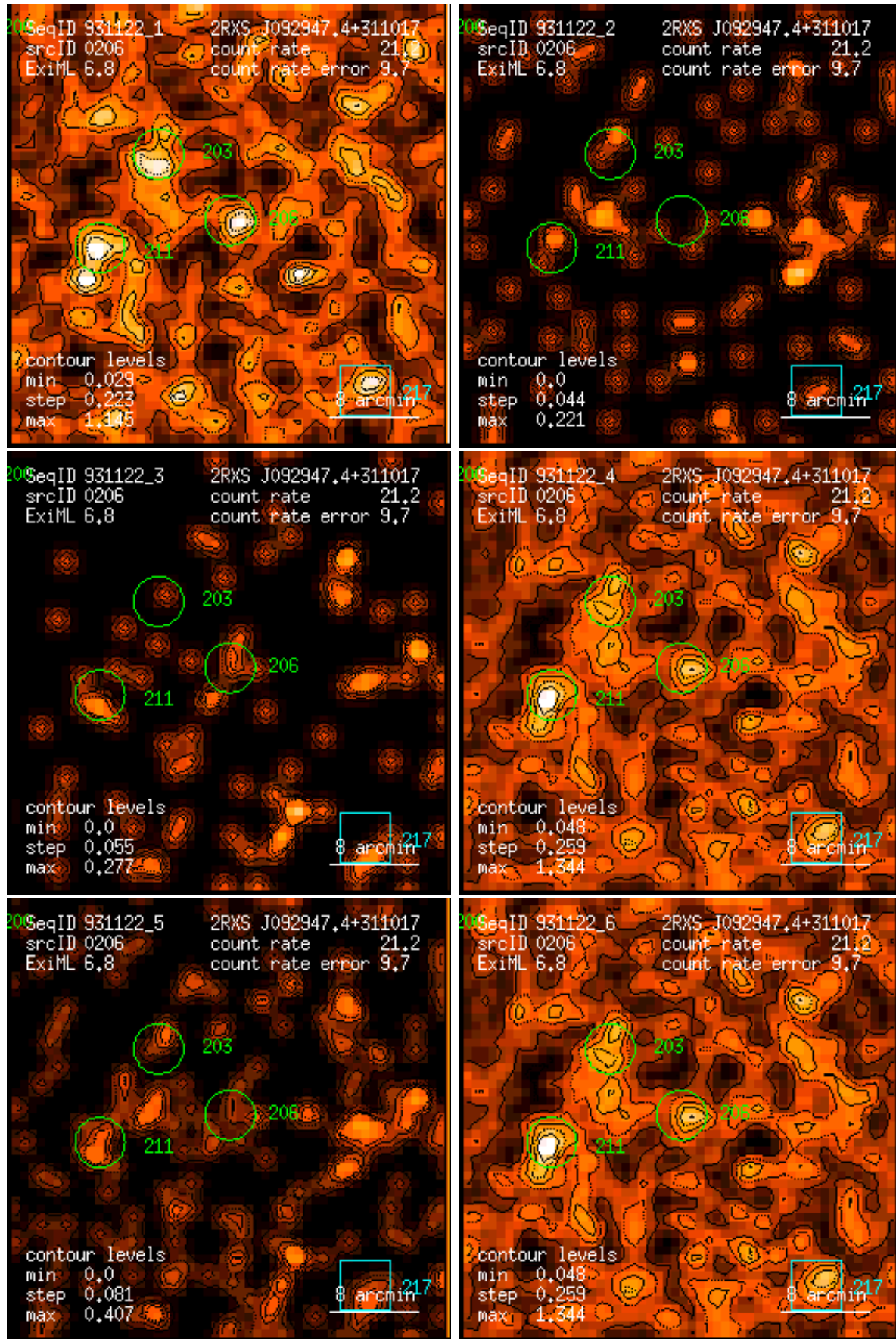
Figure 206: RASS 931122: detection 0206: band rate images, Gaussian filter: (1) PSPC channels 11 – 41, (2) 52 – 90, (3) 91 – 201, (4) 11 – 235, (5) 52 – 201, (6) 11 – 201. Broad band rates in counts/ks. Band rate contour levels in counts/ks/arcmin 2 .
