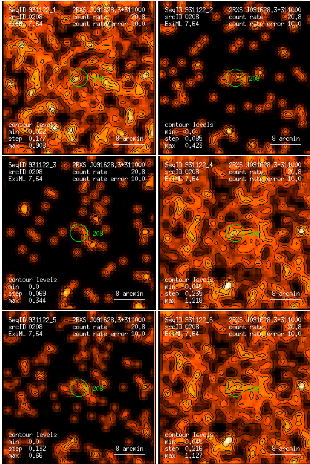
Figure 208: RASS 931122: detection 0208: band rate images, Gaussian filter: (1) PSPC channels 11 – 41, (2) 52 – 90, (3) 91 – 201, (4) 11 – 235, (5) 52 – 201, (6) 11 – 201. Broad band rates in counts/ks. Band rate contour levels in counts/ks/arcmin 2 .
