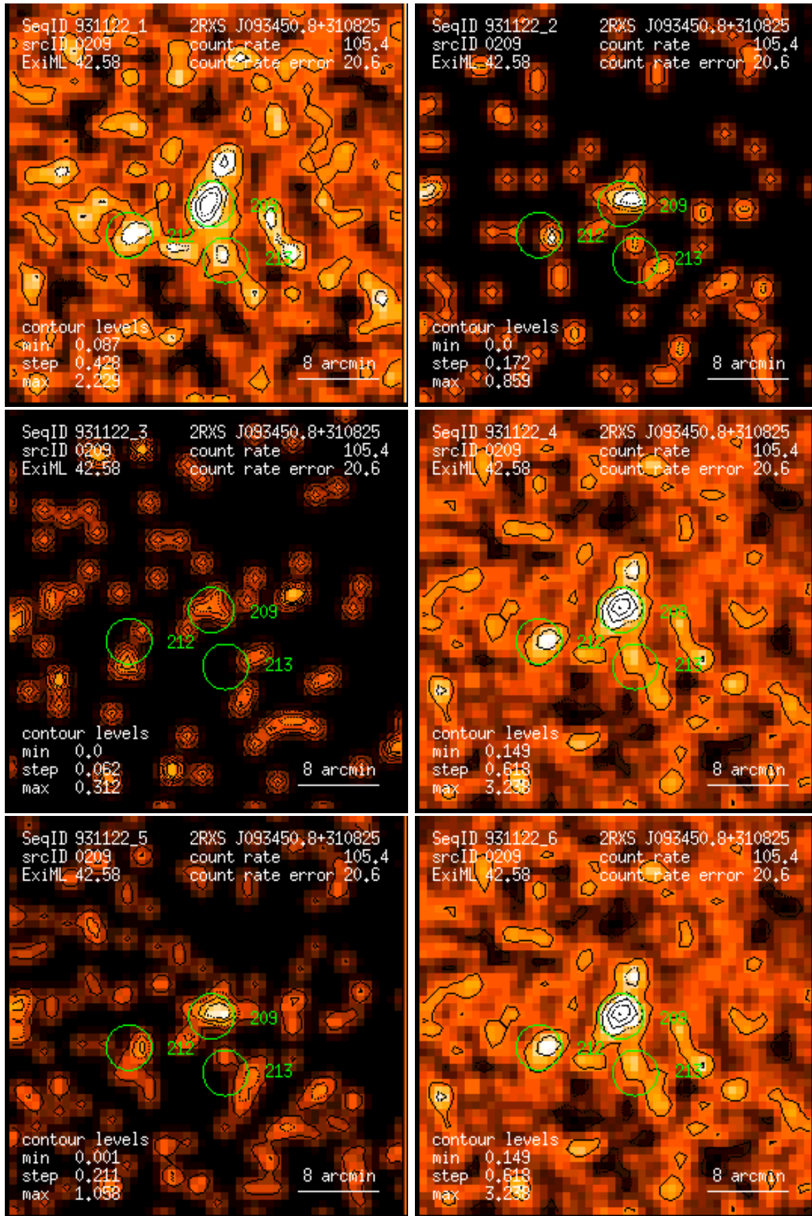
Figure 209: RASS 931122: detection 0209: band rate images, Gaussian filter: (1) PSPC channels 11 – 41, (2) 52 – 90, (3) 91 – 201, (4) 11 – 235, (5) 52 – 201, (6) 11 – 201. Broad band rates in counts/ks. Band rate contour levels in counts/ks/arcmin 2 .
