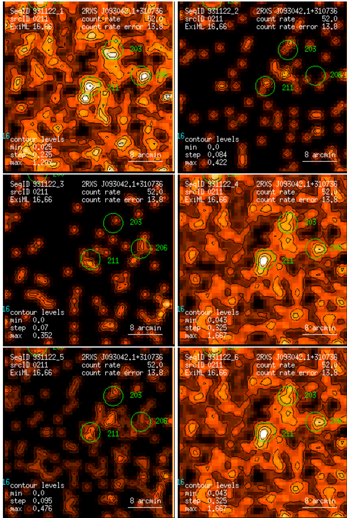
Figure 211: RASS 931122: detection 0211: band rate images, Gaussian filter: (1) PSPC channels 11 – 41, (2) 52 – 90, (3) 91 – 201, (4) 11 – 235, (5) 52 – 201, (6) 11 – 201. Broad band rates in counts/ks. Band rate contour levels in counts/ks/arcmin 2 .
