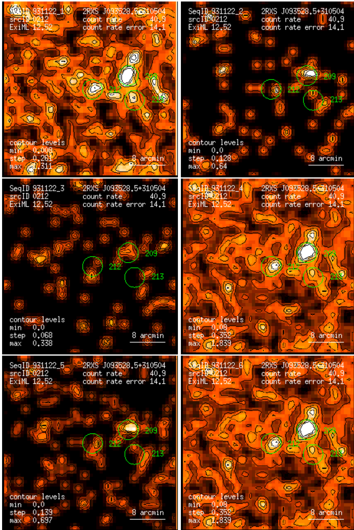
Figure 212: RASS 931122: detection 0212: band rate images, Gaussian filter: (1) PSPC channels 11 – 41, (2) 52 – 90, (3) 91 – 201, (4) 11 – 235, (5) 52 – 201, (6) 11 – 201. Broad band rates in counts/ks. Band rate contour levels in counts/ks/arcmin 2 .
