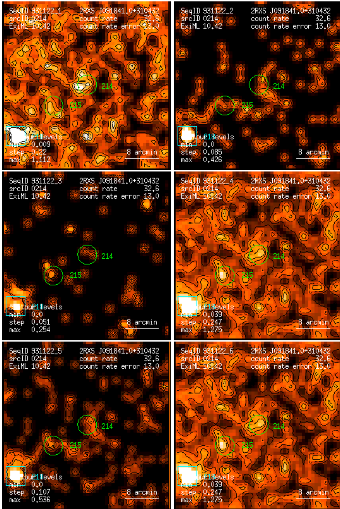
Figure 214: RASS 931122: detection 0214: band rate images, Gaussian filter: (1) PSPC channels 11 – 41, (2) 52 – 90, (3) 91 – 201, (4) 11 – 235, (5) 52 – 201, (6) 11 – 201. Broad band rates in counts/ks. Band rate contour levels in counts/ks/arcmin 2 .
