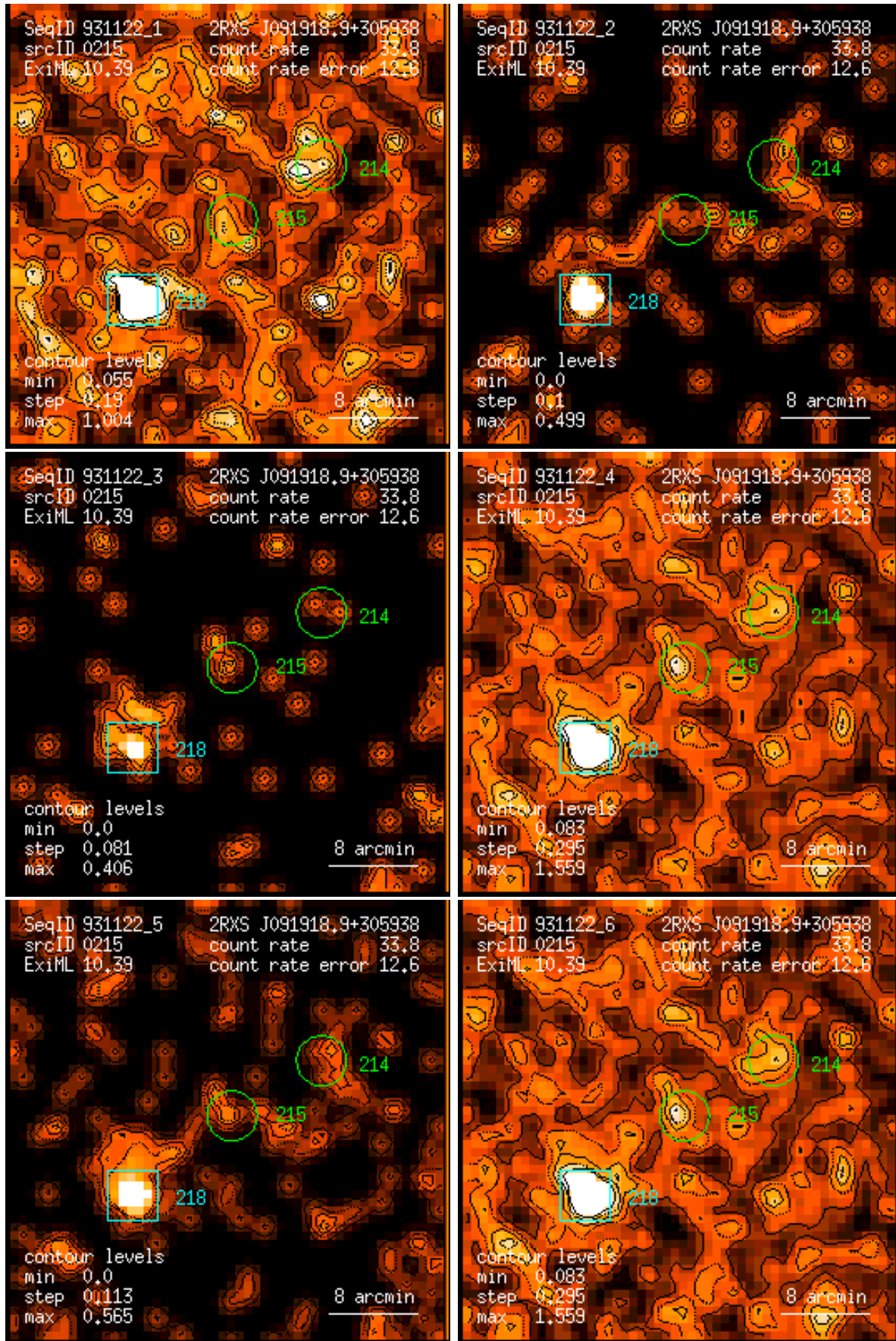
Figure 215: RASS 931122: detection 0215: band rate images, Gaussian filter: (1) PSPC channels 11 – 41, (2) 52 – 90, (3) 91 – 201, (4) 11 – 235, (5) 52 – 201, (6) 11 – 201. Broad band rates in counts/ks. Band rate contour levels in counts/ks/arcmin 2 .
