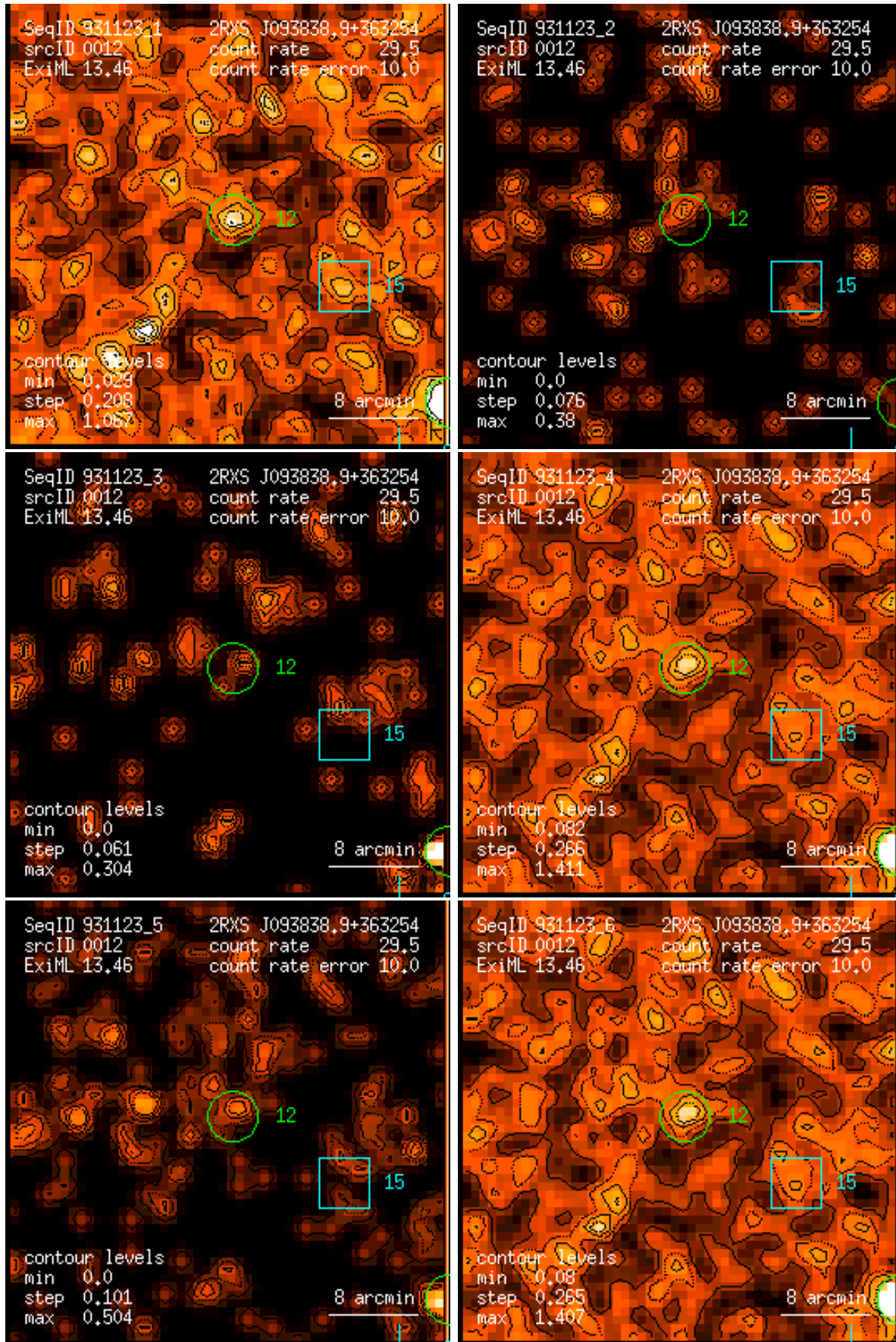
Figure 12: RASS 931123: detection 0012: band rate images, Gaussian filter: (1) PSPC channels 11 – 41, (2) 52 – 90, (3) 91 – 201, (4) 11 – 235, (5) 52 – 201, (6) 11 – 201. Broad band rates in counts/ks. Band rate contour levels in counts/ks/arcmin 2 .
