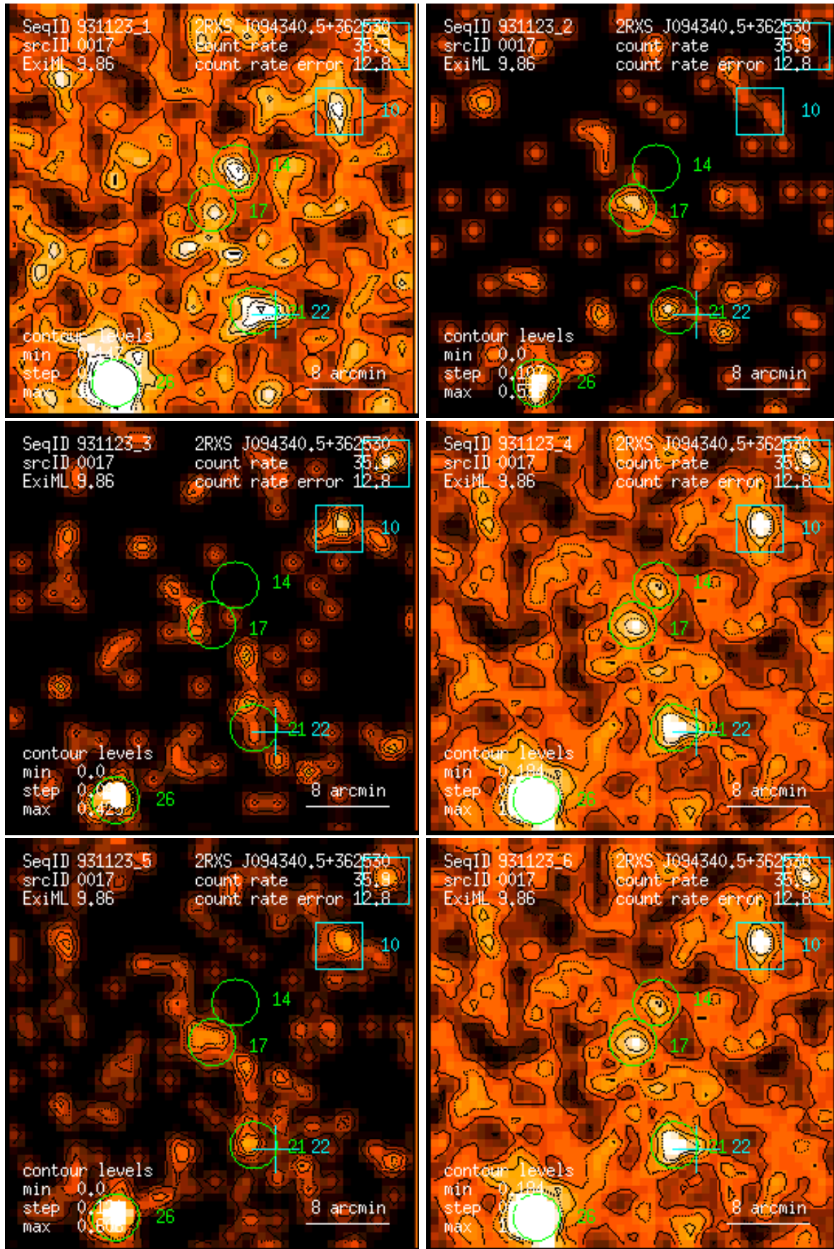
Figure 17: RASS 931123: detection 0017: band rate images, Gaussian filter: (1) PSPC channels 11 – 41, (2) 52 – 90, (3) 91 – 201, (4) 11 – 235, (5) 52 – 201, (6) 11 – 201. Broad band rates in counts/ks. Band rate contour levels in counts/ks/arcmin 2 .
