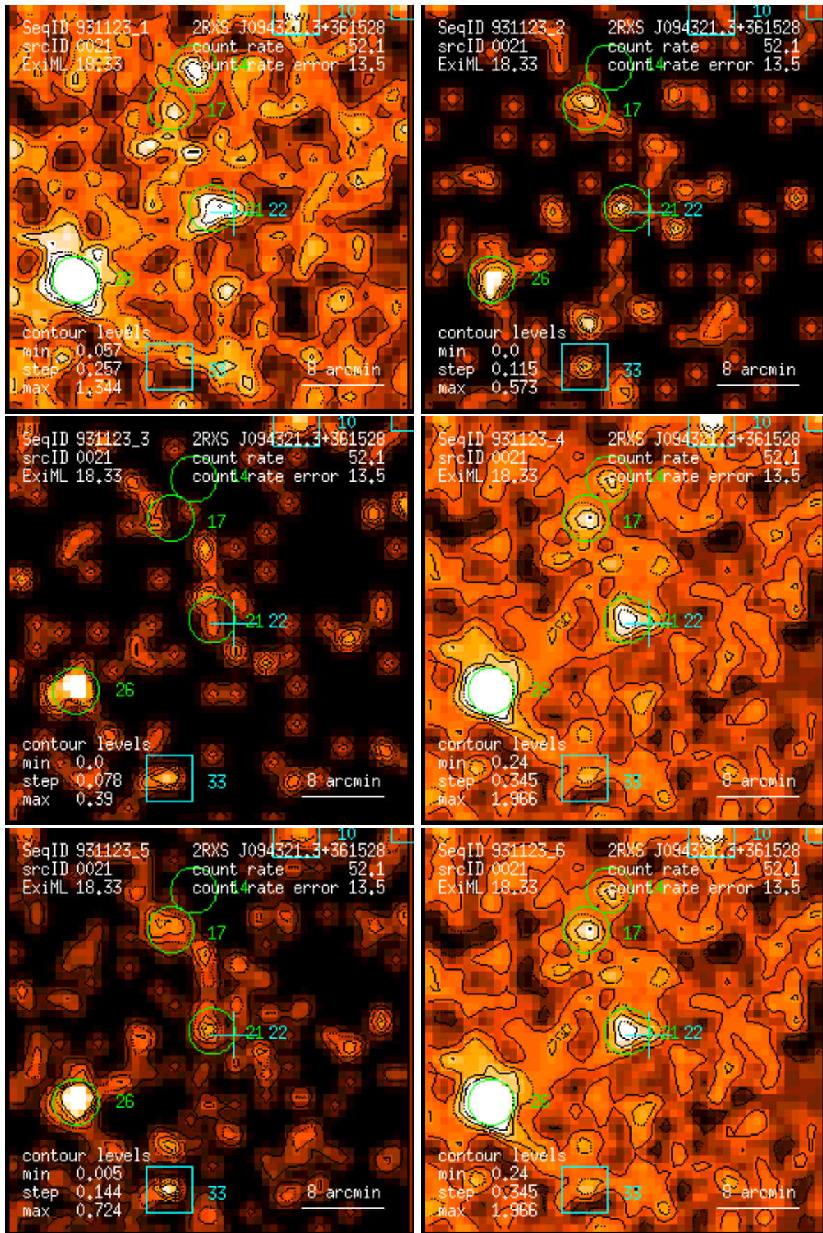
Figure 21: RASS 931123: detection 0021: band rate images, Gaussian filter: (1) PSPC channels 11 – 41, (2) 52 – 90, (3) 91 – 201, (4) 11 – 235, (5) 52 – 201, (6) 11 – 201. Broad band rates in counts/ks. Band rate contour levels in counts/ks/arcmin 2 .
