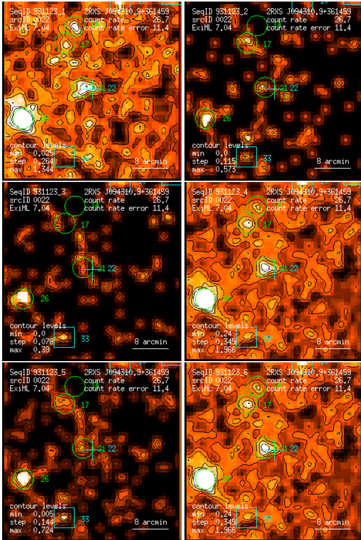
Figure 22: RASS 931123: detection 0022: band rate images, Gaussian filter: (1) PSPC channels 11 – 41, (2) 52 – 90, (3) 91 – 201, (4) 11 – 235, (5) 52 – 201, (6) 11 – 201. Broad band rates in counts/ks. Band rate contour levels in counts/ks/arcmin 2 .
