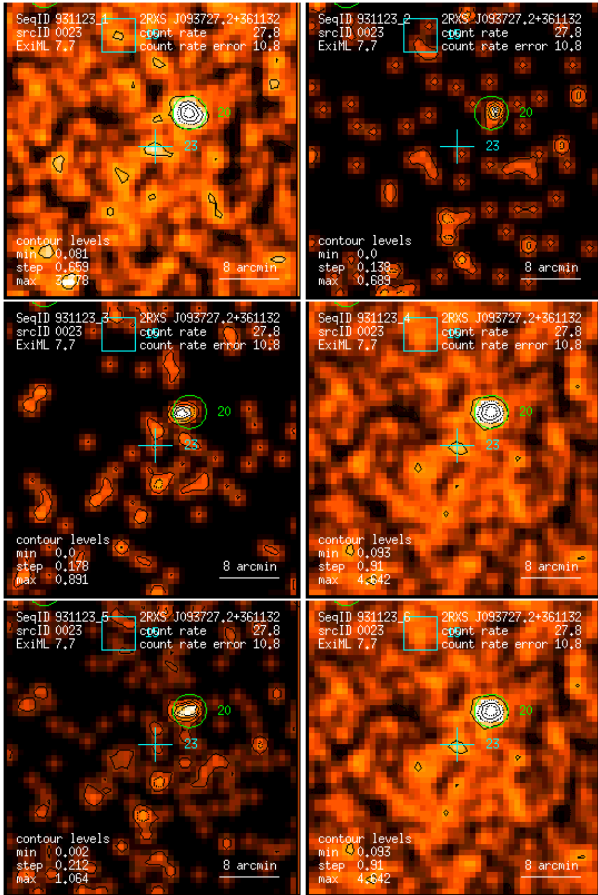
Figure 23: RASS 931123: detection 0023: band rate images, Gaussian filter: (1) PSPC channels 11 – 41, (2) 52 – 90, (3) 91 – 201, (4) 11 – 235, (5) 52 – 201, (6) 11 – 201. Broad band rates in counts/ks. Band rate contour levels in counts/ks/arcmin 2 .
