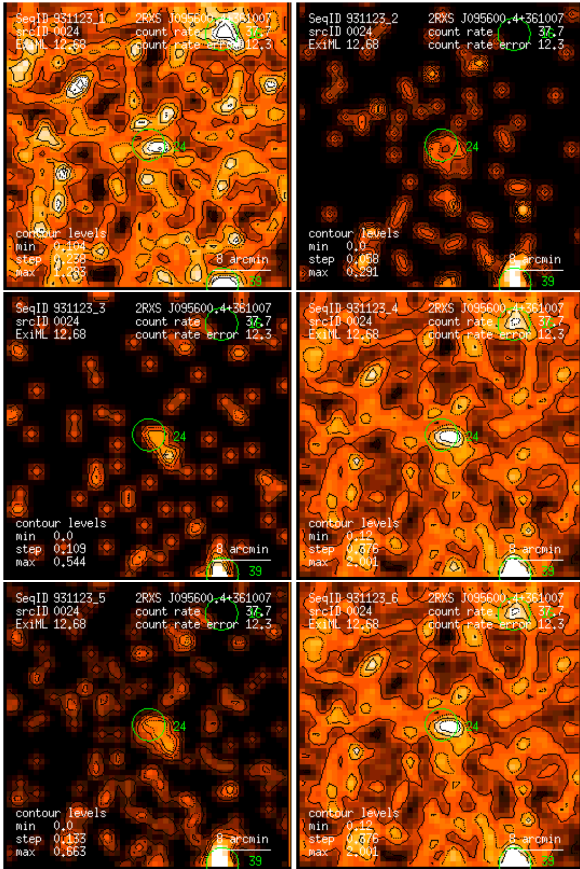
Figure 24: RASS 931123: detection 0024: band rate images, Gaussian filter: (1) PSPC channels 11 – 41, (2) 52 – 90, (3) 91 – 201, (4) 11 – 235, (5) 52 – 201, (6) 11 – 201. Broad band rates in counts/ks. Band rate contour levels in counts/ks/arcmin 2 .
