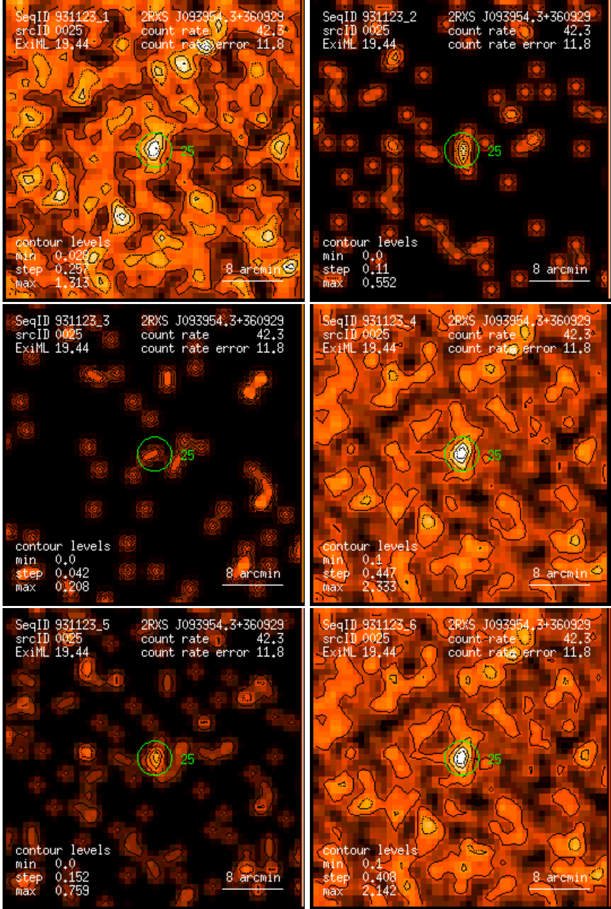
Figure 25: RASS 931123: detection 0025: band rate images, Gaussian filter: (1) PSPC channels 11 – 41, (2) 52 – 90, (3) 91 – 201, (4) 11 – 235, (5) 52 – 201, (6) 11 – 201. Broad band rates in counts/ks. Band rate contour levels in counts/ks/arcmin 2 .
