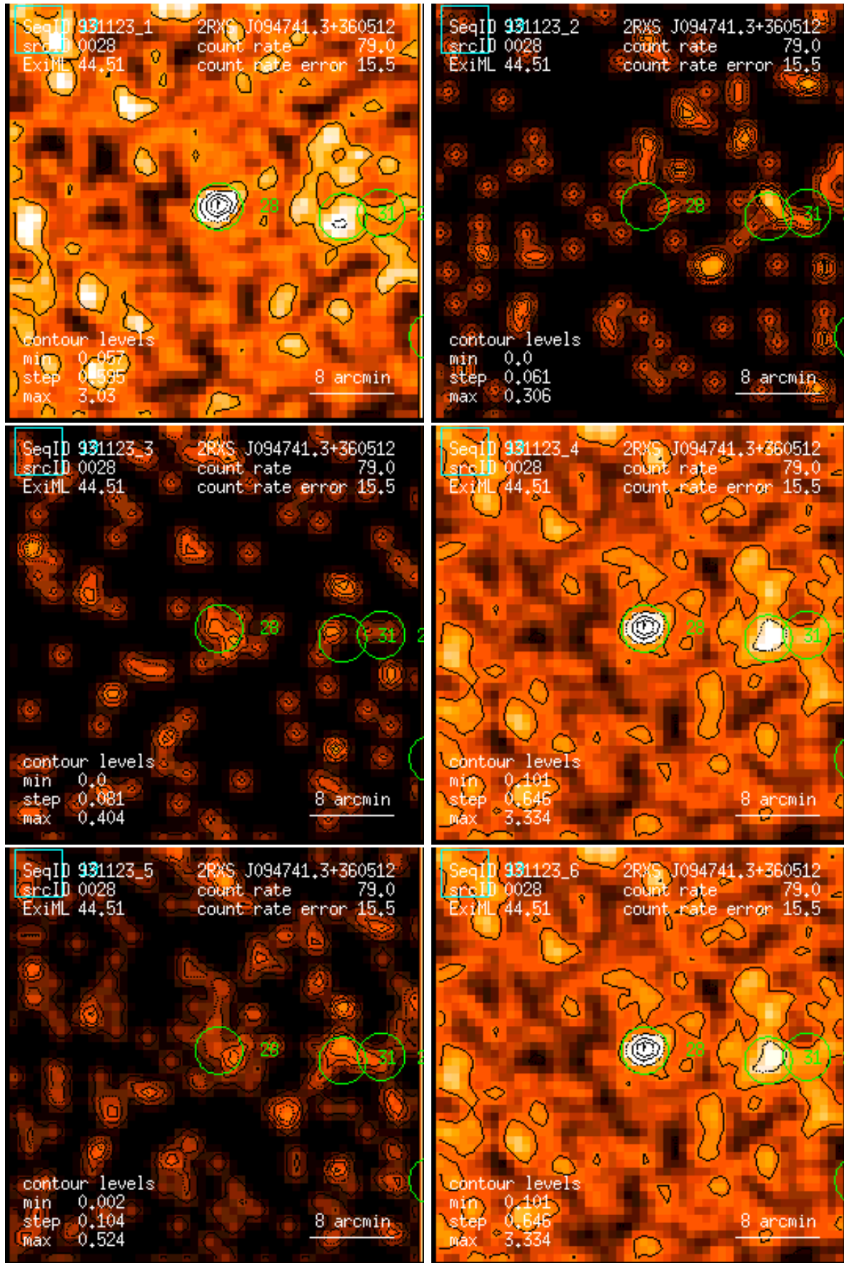
Figure 28: RASS 931123: detection 0028: band rate images, Gaussian filter: (1) PSPC channels 11 – 41, (2) 52 – 90, (3) 91 – 201, (4) 11 – 235, (5) 52 – 201, (6) 11 – 201. Broad band rates in counts/ks. Band rate contour levels in counts/ks/arcmin 2 .
