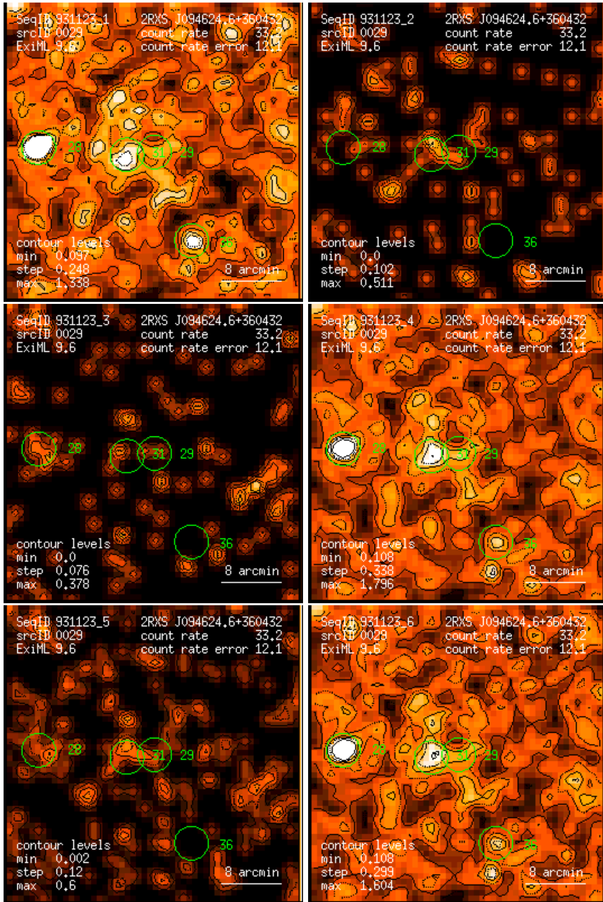
Figure 29: RASS 931123: detection 0029: band rate images, Gaussian filter: (1) PSPC channels 11 – 41, (2) 52 – 90, (3) 91 – 201, (4) 11 – 235, (5) 52 – 201, (6) 11 – 201. Broad band rates in counts/ks. Band rate contour levels in counts/ks/arcmin 2 .
