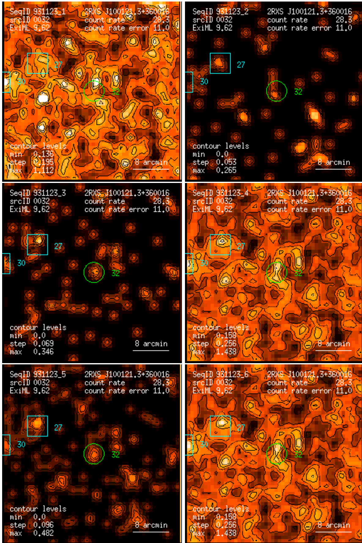
Figure 32: RASS 931123: detection 0032: band rate images, Gaussian filter: (1) PSPC channels 11 – 41, (2) 52 – 90, (3) 91 – 201, (4) 11 – 235, (5) 52 – 201, (6) 11 – 201. Broad band rates in counts/ks. Band rate contour levels in counts/ks/arcmin 2 .
