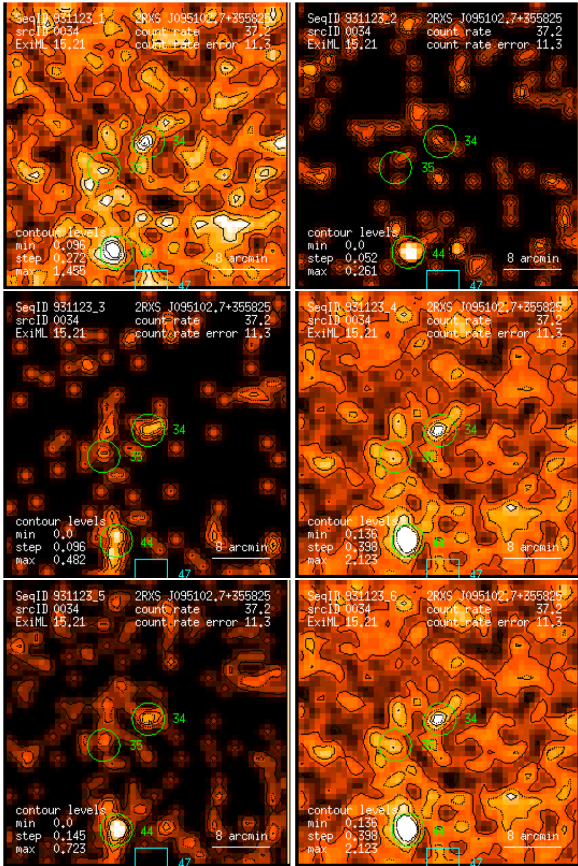
Figure 34: RASS 931123: detection 0034: band rate images, Gaussian filter: (1) PSPC channels 11 – 41, (2) 52 – 90, (3) 91 – 201, (4) 11 – 235, (5) 52 – 201, (6) 11 – 201. Broad band rates in counts/ks. Band rate contour levels in counts/ks/arcmin 2 .
