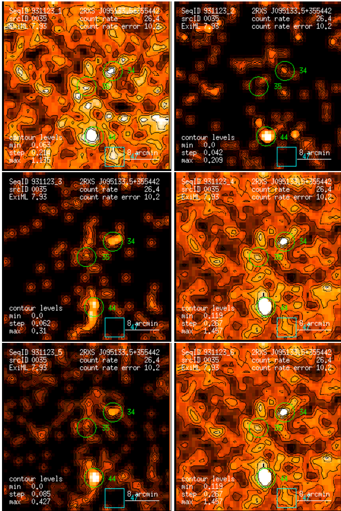
Figure 35: RASS 931123: detection 0035: band rate images, Gaussian filter: (1) PSPC channels 11 – 41, (2) 52 – 90, (3) 91 – 201, (4) 11 – 235, (5) 52 – 201, (6) 11 – 201. Broad band rates in counts/ks. Band rate contour levels in counts/ks/arcmin 2 .
