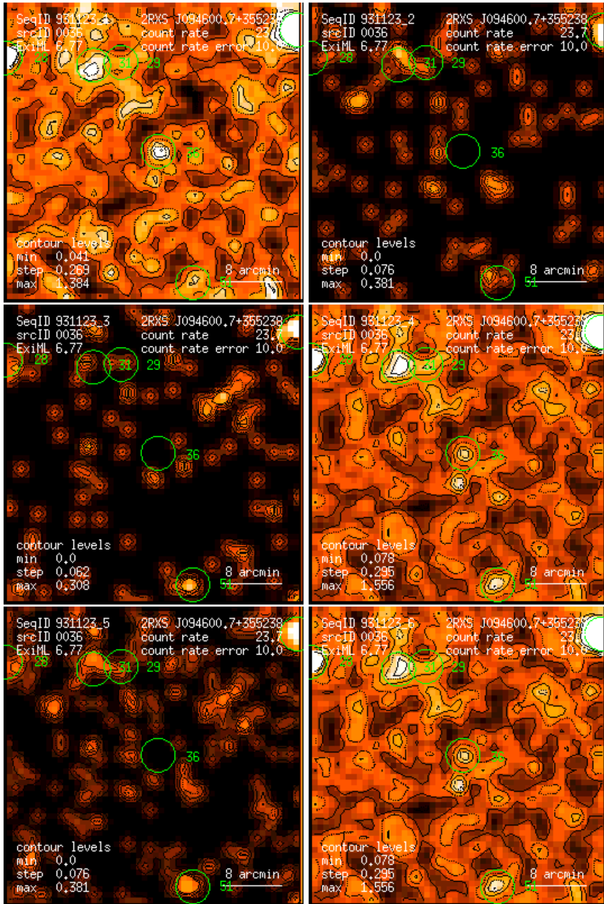
Figure 36: RASS 931123: detection 0036: band rate images, Gaussian filter: (1) PSPC channels 11 – 41, (2) 52 – 90, (3) 91 – 201, (4) 11 – 235, (5) 52 – 201, (6) 11 – 201. Broad band rates in counts/ks. Band rate contour levels in counts/ks/arcmin 2 .
