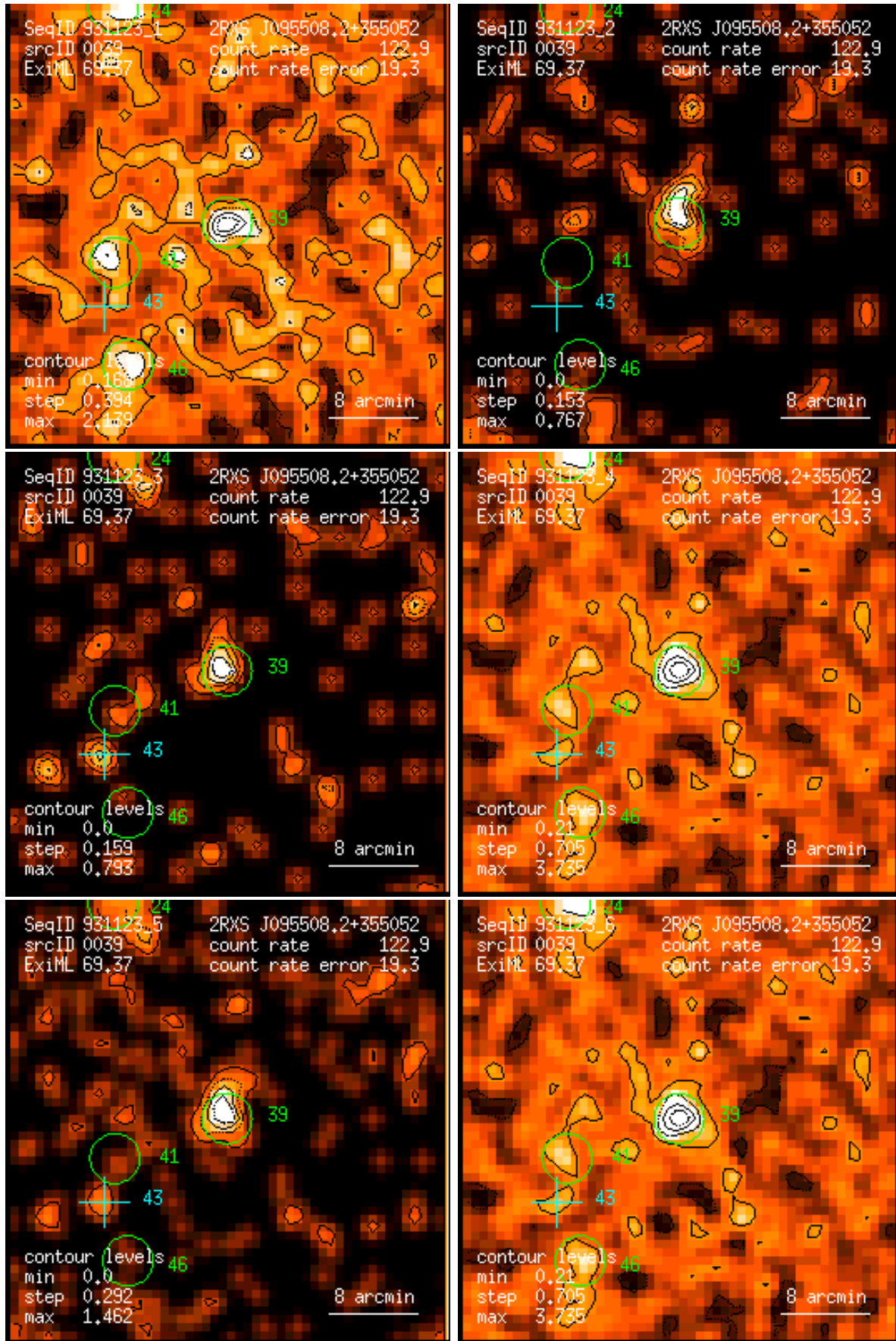
Figure 39: RASS 931123: detection 0039: band rate images, Gaussian filter: (1) PSPC channels 11 – 41, (2) 52 – 90, (3) 91 – 201, (4) 11 – 235, (5) 52 – 201, (6) 11 – 201. Broad band rates in counts/ks. Band rate contour levels in counts/ks/arcmin 2 .
