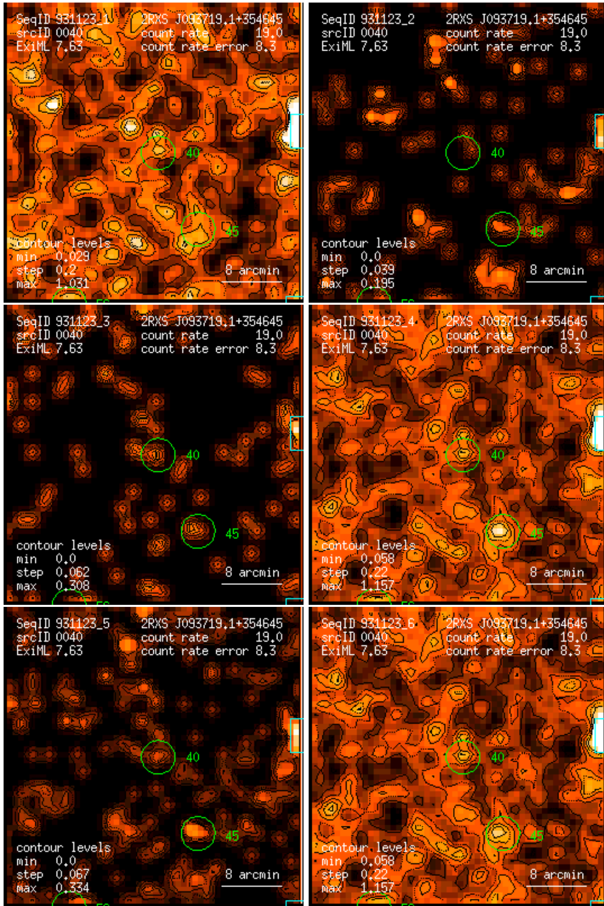
Figure 40: RASS 931123: detection 0040: band rate images, Gaussian filter: (1) PSPC channels 11 – 41, (2) 52 – 90, (3) 91 – 201, (4) 11 – 235, (5) 52 – 201, (6) 11 – 201. Broad band rates in counts/ks. Band rate contour levels in counts/ks/arcmin 2 .
