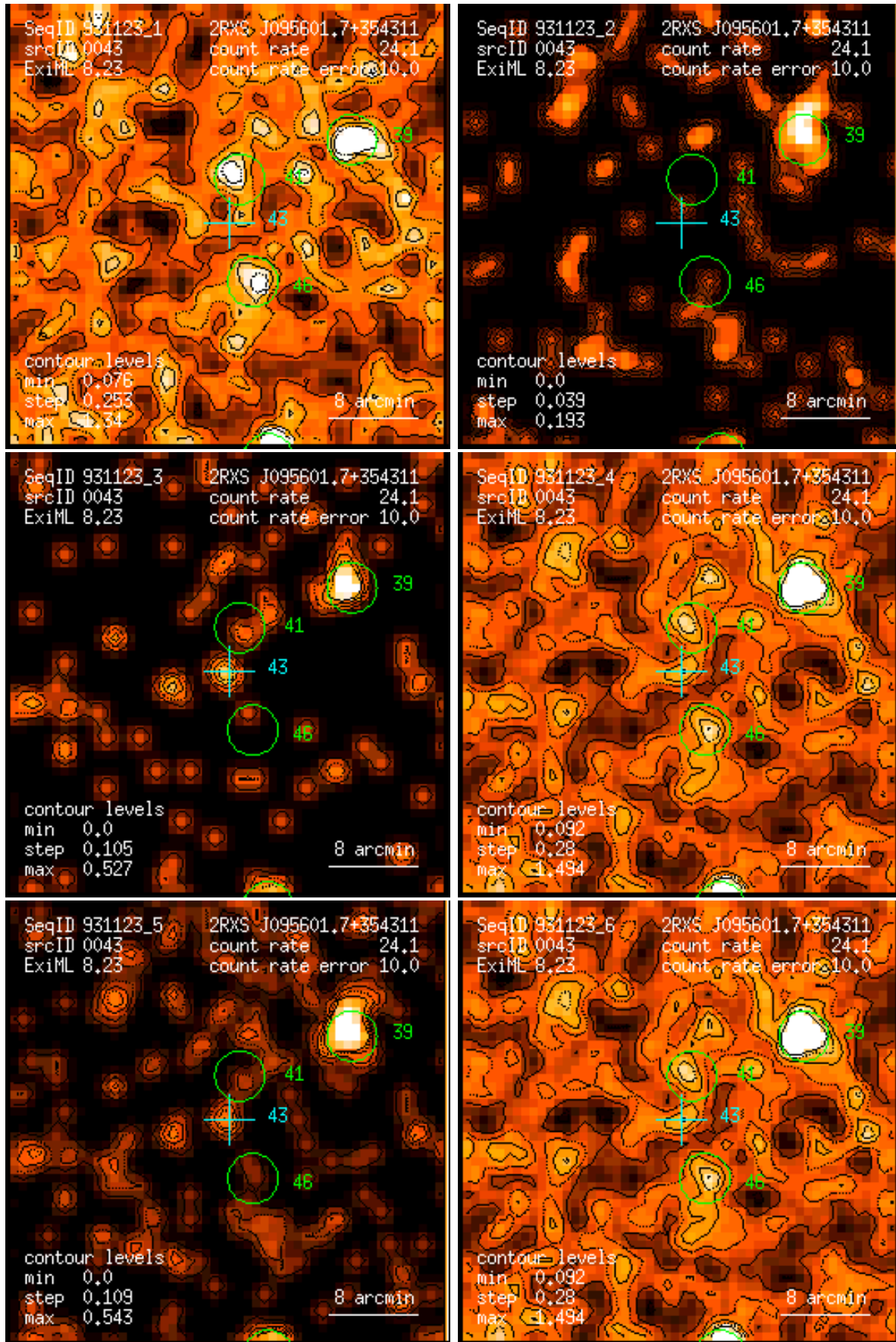
Figure 43: RASS 931123: detection 0043: band rate images, Gaussian filter: (1) PSPC channels 11 – 41, (2) 52 – 90, (3) 91 – 201, (4) 11 – 235, (5) 52 – 201, (6) 11 – 201. Broad band rates in counts/ks. Band rate contour levels in counts/ks/arcmin 2 .
