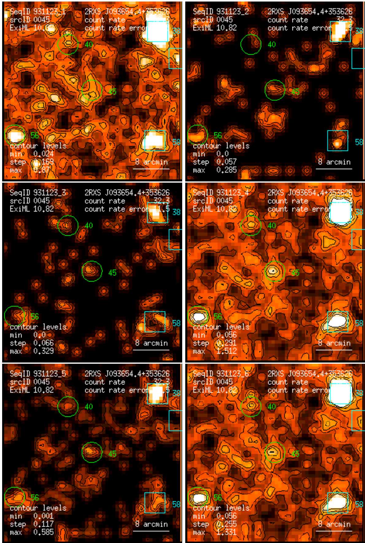
Figure 45: RASS 931123: detection 0045: band rate images, Gaussian filter: (1) PSPC channels 11 – 41, (2) 52 – 90, (3) 91 – 201, (4) 11 – 235, (5) 52 – 201, (6) 11 – 201. Broad band rates in counts/ks. Band rate contour levels in counts/ks/arcmin 2 .
