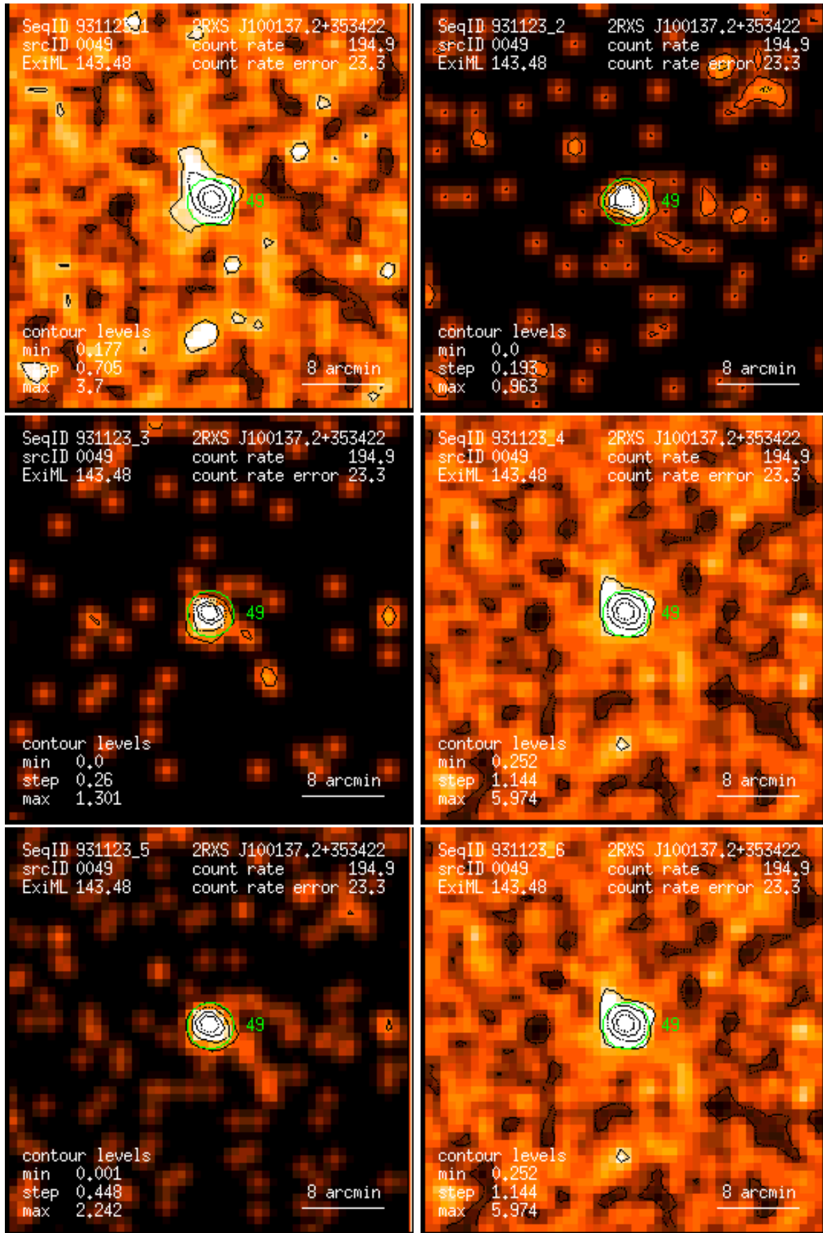
Figure 49: RASS 931123: detection 0049: band rate images, Gaussian filter: (1) PSPC channels 11 – 41, (2) 52 – 90, (3) 91 – 201, (4) 11 – 235, (5) 52 – 201, (6) 11 – 201. Broad band rates in counts/ks. Band rate contour levels in counts/ks/arcmin 2 .
