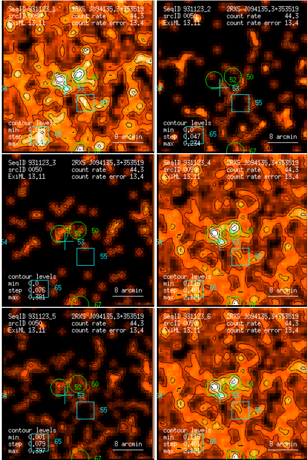
Figure 50: RASS 931123: detection 0050: band rate images, Gaussian filter: (1) PSPC channels 11 – 41, (2) 52 – 90, (3) 91 – 201, (4) 11 – 235, (5) 52 – 201, (6) 11 – 201. Broad band rates in counts/ks. Band rate contour levels in counts/ks/arcmin 2 .
