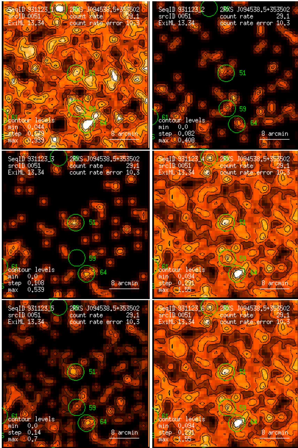
Figure 51: RASS 931123: detection 0051: band rate images, Gaussian filter: (1) PSPC channels 11 – 41, (2) 52 – 90, (3) 91 – 201, (4) 11 – 235, (5) 52 – 201, (6) 11 – 201. Broad band rates in counts/ks. Band rate contour levels in counts/ks/arcmin 2 .
