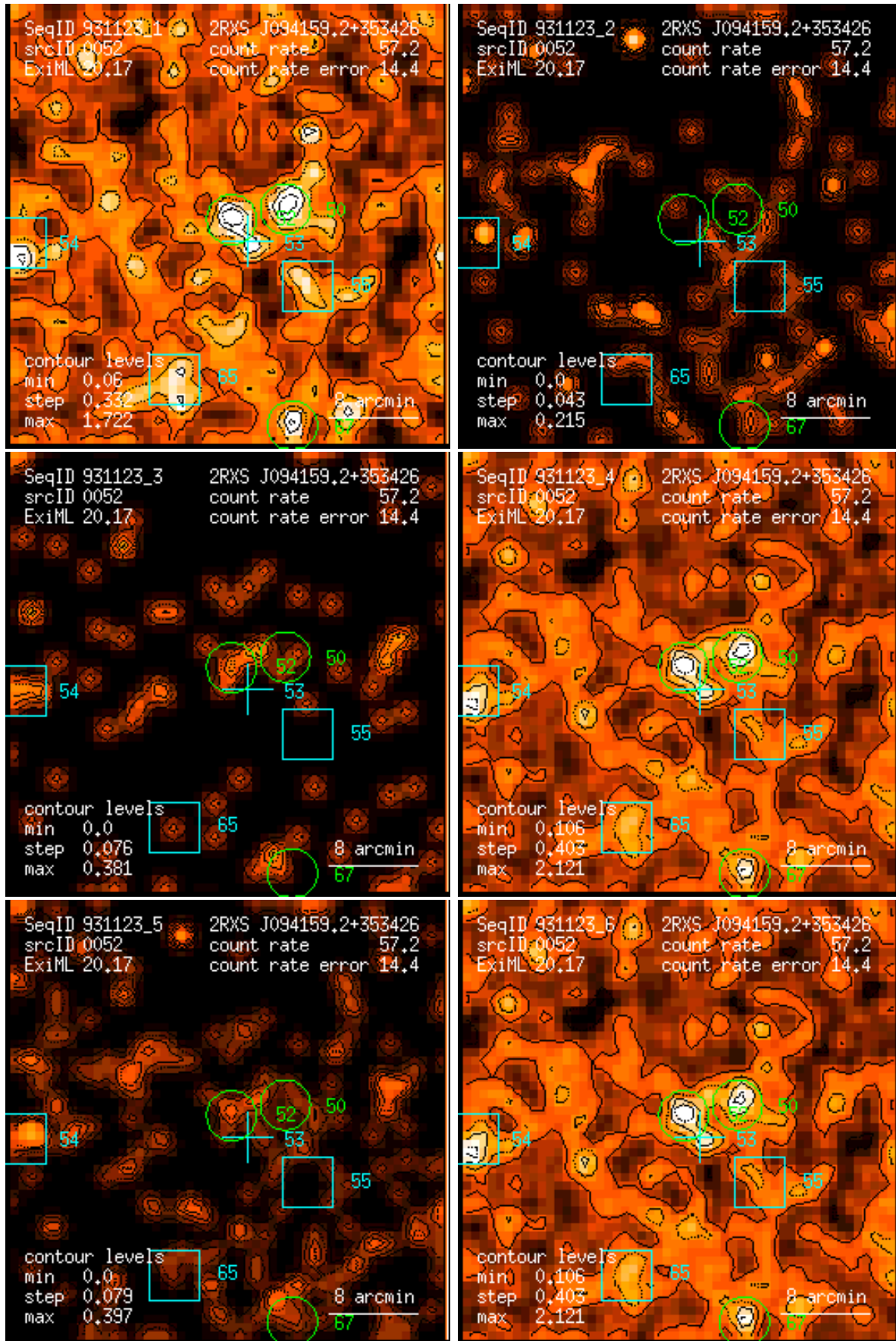
Figure 52: RASS 931123: detection 0052: band rate images, Gaussian filter: (1) PSPC channels 11 – 41, (2) 52 – 90, (3) 91 – 201, (4) 11 – 235, (5) 52 – 201, (6) 11 – 201. Broad band rates in counts/ks. Band rate contour levels in counts/ks/arcmin 2 .
