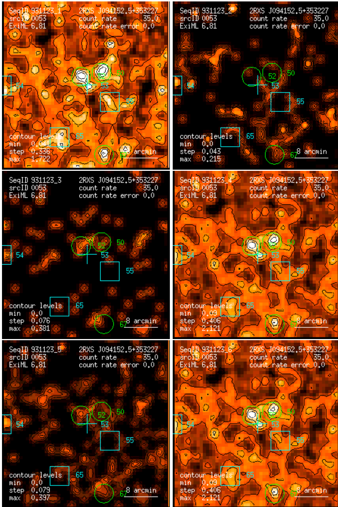
Figure 53: RASS 931123: detection 0053: band rate images, Gaussian filter: (1) PSPC channels 11 – 41, (2) 52 – 90, (3) 91 – 201, (4) 11 – 235, (5) 52 – 201, (6) 11 – 201. Broad band rates in counts/ks. Band rate contour levels in counts/ks/arcmin 2 .
