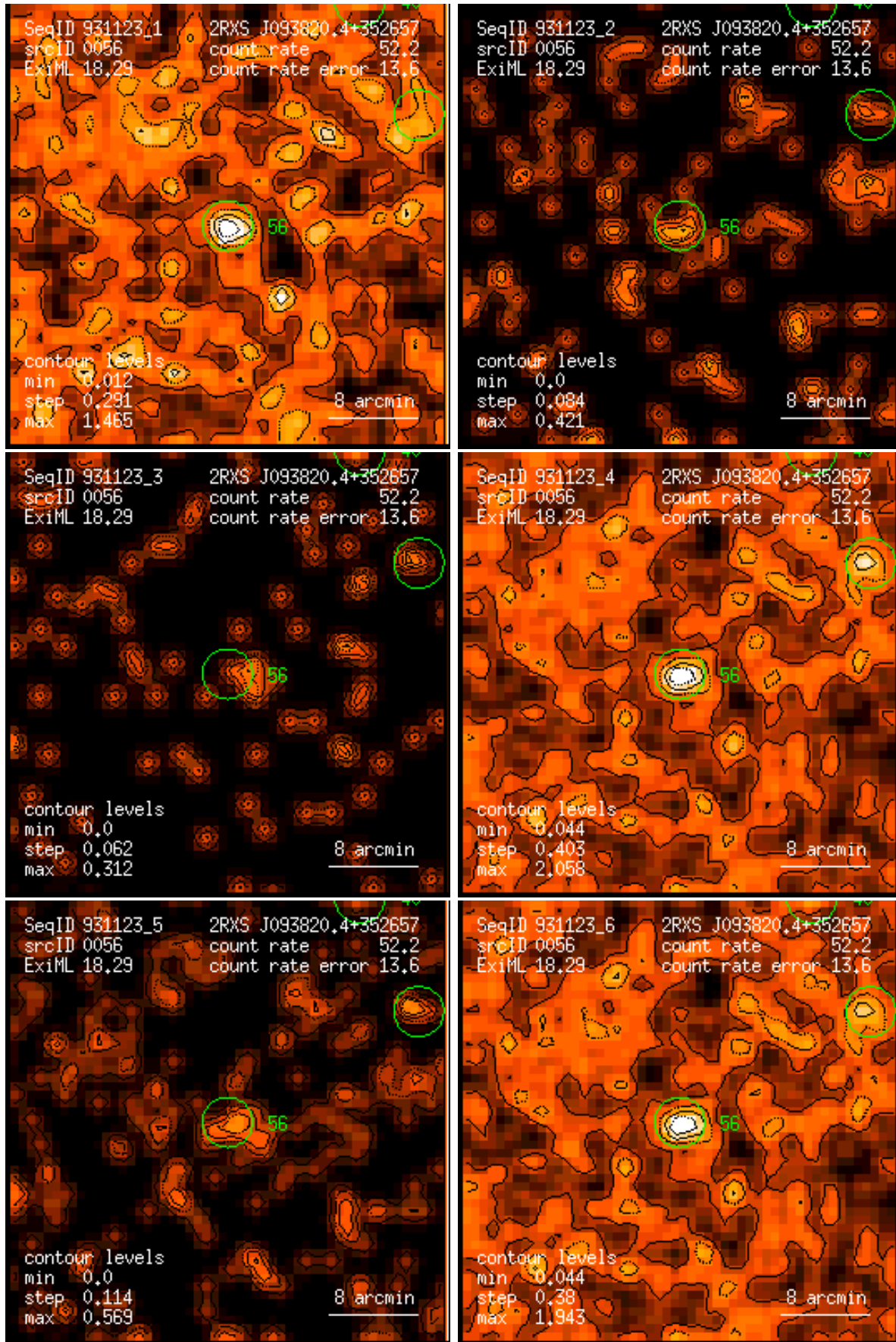
Figure 56: RASS 931123: detection 0056: band rate images, Gaussian filter: (1) PSPC channels 11 – 41, (2) 52 – 90, (3) 91 – 201, (4) 11 – 235, (5) 52 – 201, (6) 11 – 201. Broad band rates in counts/ks. Band rate contour levels in counts/ks/arcmin 2 .
