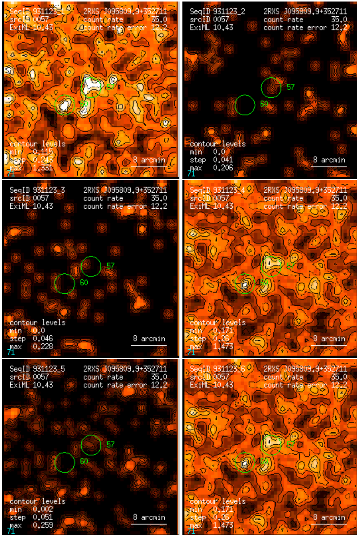
Figure 57: RASS 931123: detection 0057: band rate images, Gaussian filter: (1) PSPC channels 11 – 41, (2) 52 – 90, (3) 91 – 201, (4) 11 – 235, (5) 52 – 201, (6) 11 – 201. Broad band rates in counts/ks. Band rate contour levels in counts/ks/arcmin 2 .
