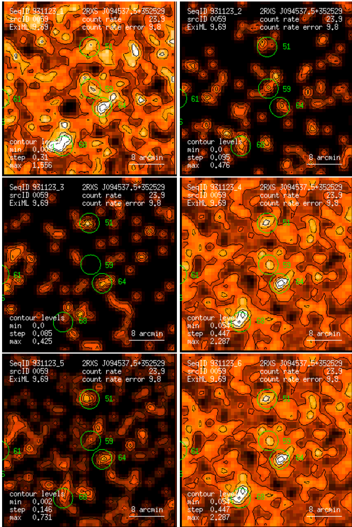
Figure 59: RASS 931123: detection 0059: band rate images, Gaussian filter: (1) PSPC channels 11 – 41, (2) 52 – 90, (3) 91 – 201, (4) 11 – 235, (5) 52 – 201, (6) 11 – 201. Broad band rates in counts/ks. Band rate contour levels in counts/ks/arcmin 2 .
