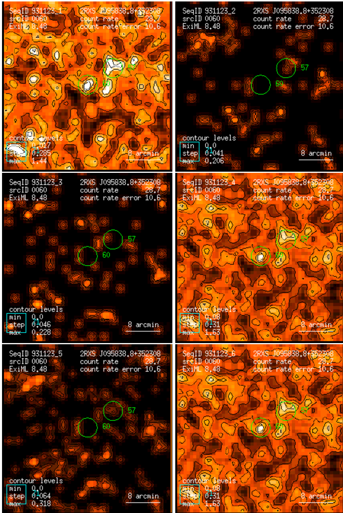
Figure 60: RASS 931123: detection 0060: band rate images, Gaussian filter: (1) PSPC channels 11 – 41, (2) 52 – 90, (3) 91 – 201, (4) 11 – 235, (5) 52 – 201, (6) 11 – 201. Broad band rates in counts/ks. Band rate contour levels in counts/ks/arcmin 2 .
