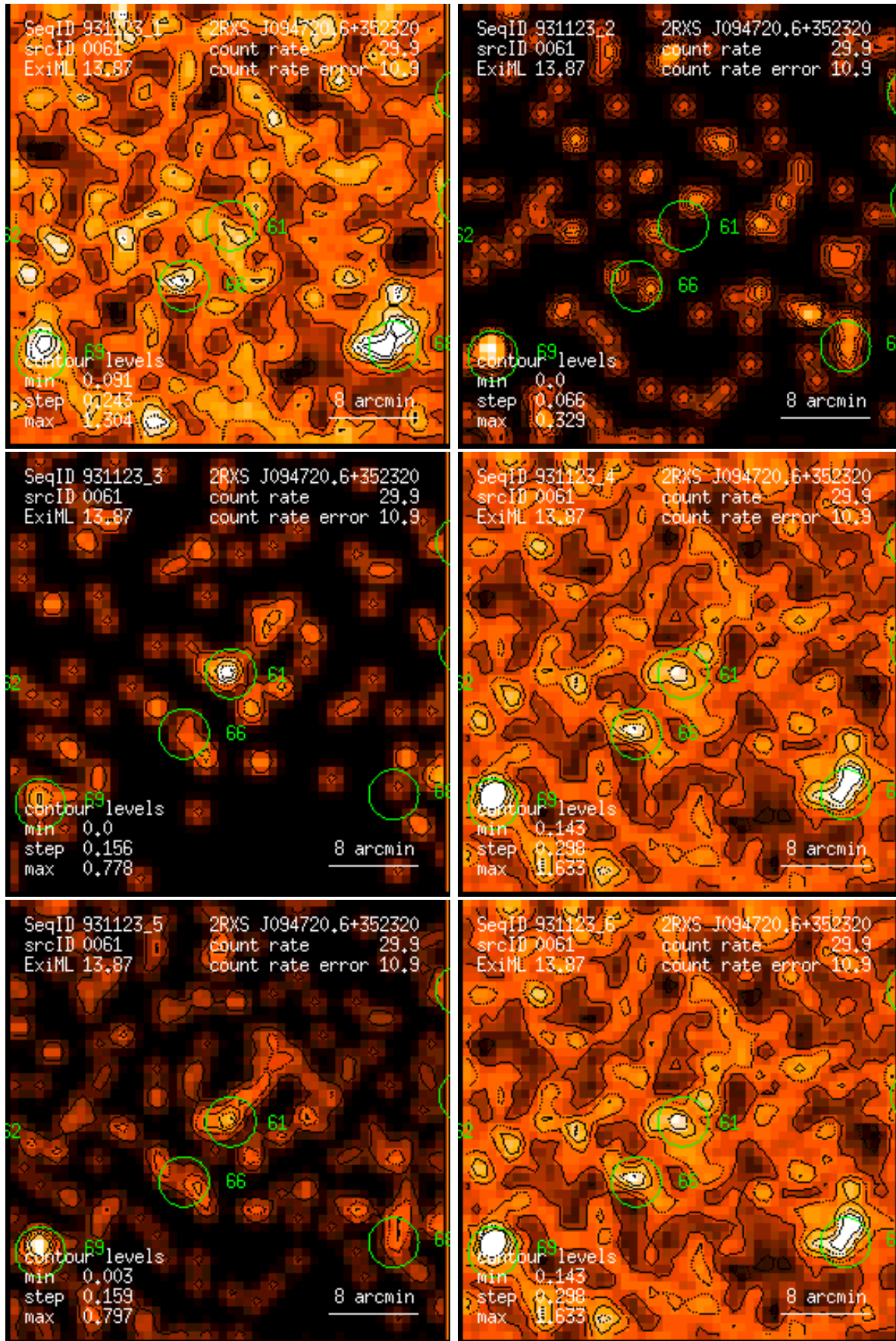
Figure 61: RASS 931123: detection 0061: band rate images, Gaussian filter: (1) PSPC channels 11 – 41, (2) 52 – 90, (3) 91 – 201, (4) 11 – 235, (5) 52 – 201, (6) 11 – 201. Broad band rates in counts/ks. Band rate contour levels in counts/ks/arcmin 2 .
